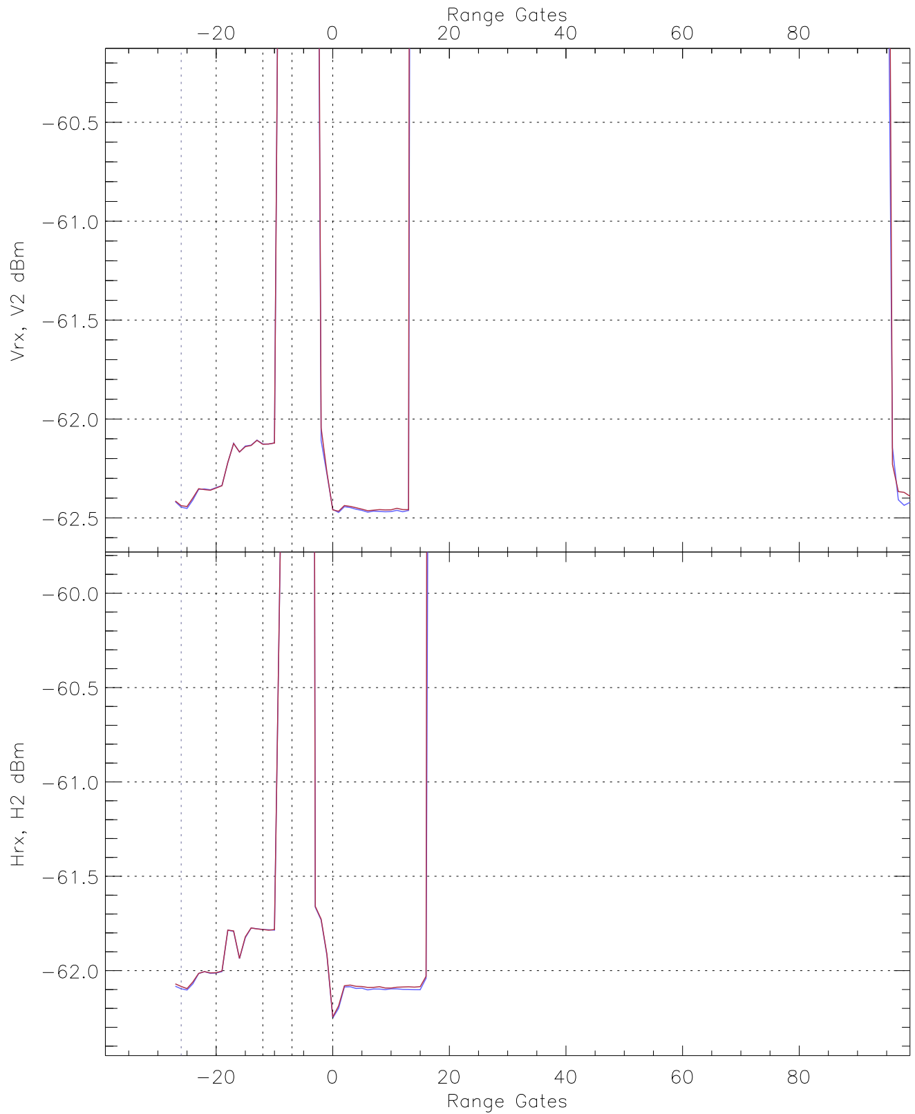
WCR2 CPP Averaged Received power for the negative gates and up to 100 gates blue: 193851-194821, 11401 profiles averaged red: 194821-195751, 11400 profiles averaged
