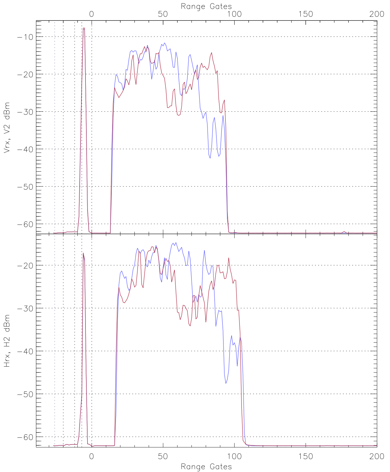
WCR2 CPP Averaged Received power for all recorded gates blue: 193851-194821, 11401 profiles averaged red: 194821-195751, 11400 profiles averaged
