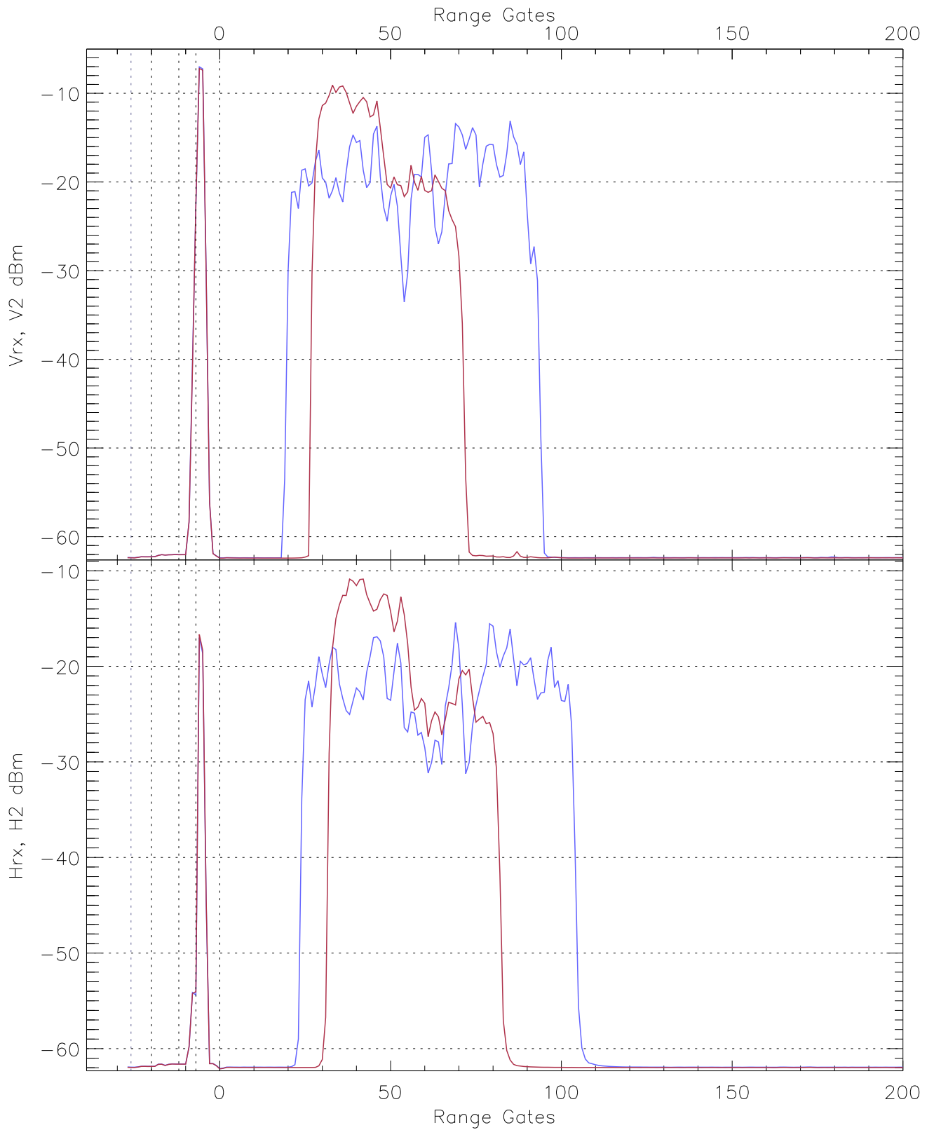
WCR2 CPP Averaged Received power for all recorded gates blue: 174020-175048, 12569 profiles averaged red: 175048-180117, 12569 profiles averaged
