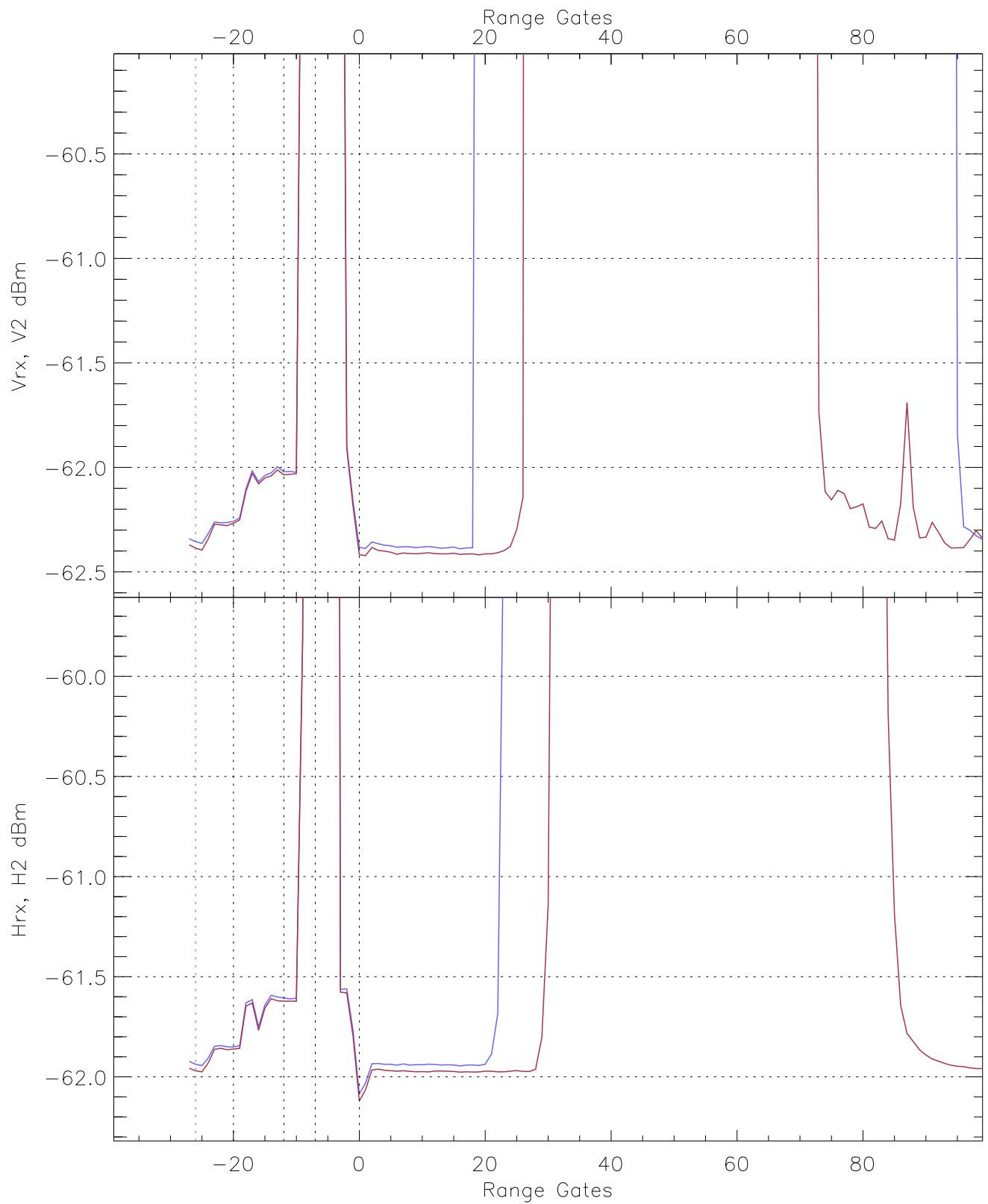
WCR2 CPP Averaged Received power for the negative gates and up to 100 gates blue: 174020-175048, 12569 profiles averaged red: 175048-180117, 12569 profiles averaged
