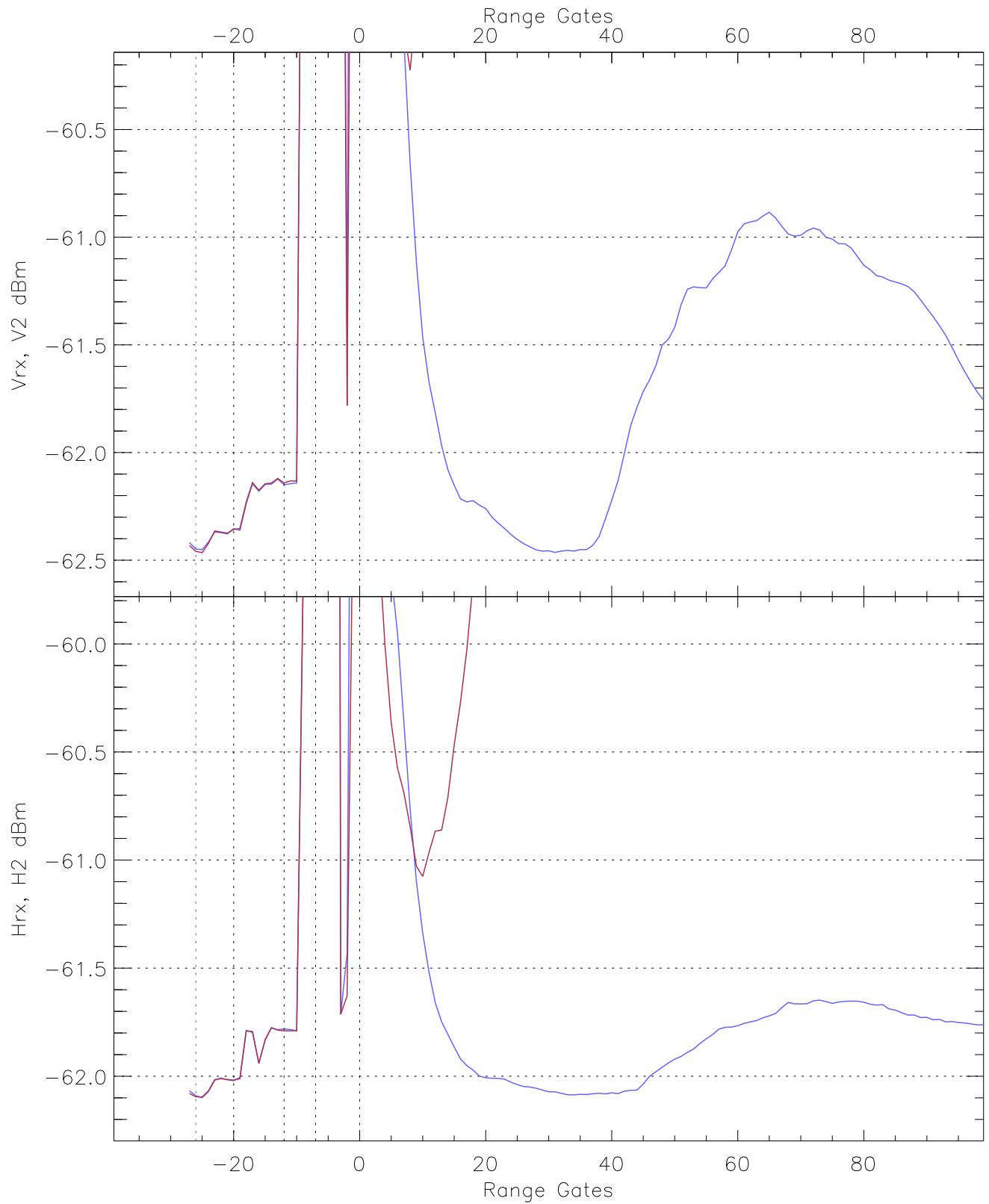
WCR2 CPP Averaged Received power for the negative gates and up to 100 gates blue: 181500-181955, 5917 profiles averaged red: 181955-182451, 5917 profiles averaged
