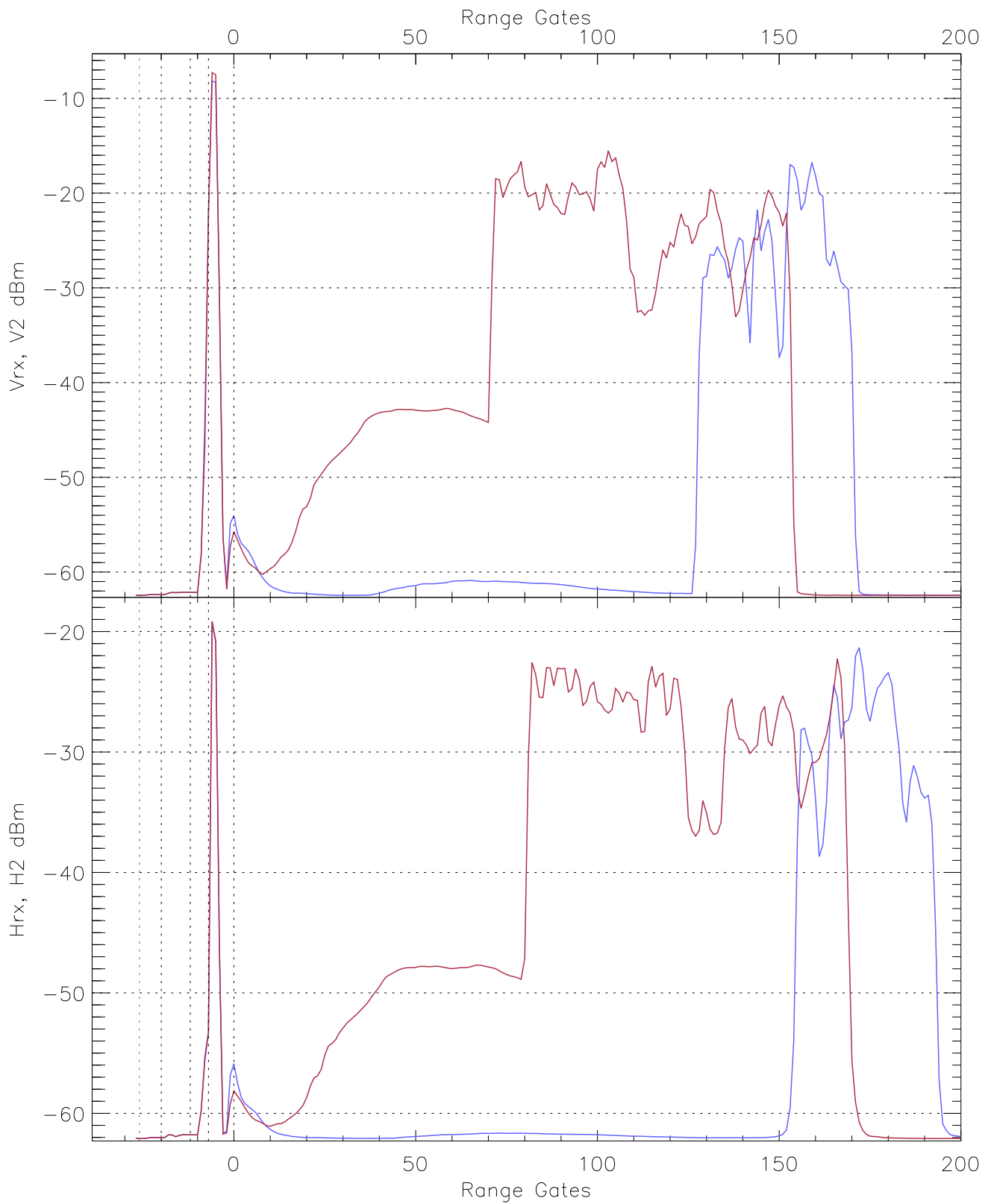
WCR2 CPP Averaged Received power for all recorded gates blue: 181500-181955, 5917 profiles averaged red: 181955-182451, 5917 profiles averaged
