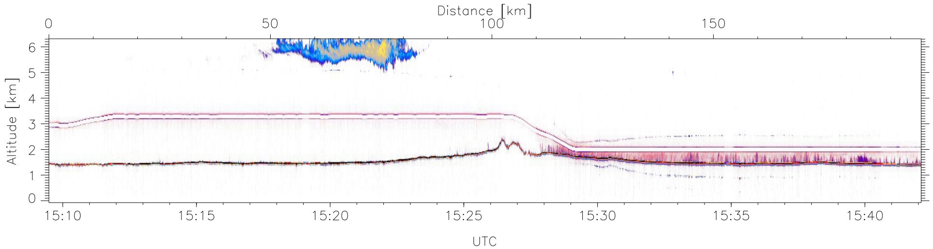
W2009-06-05-15-09-29, Up and Down Reflectivity
