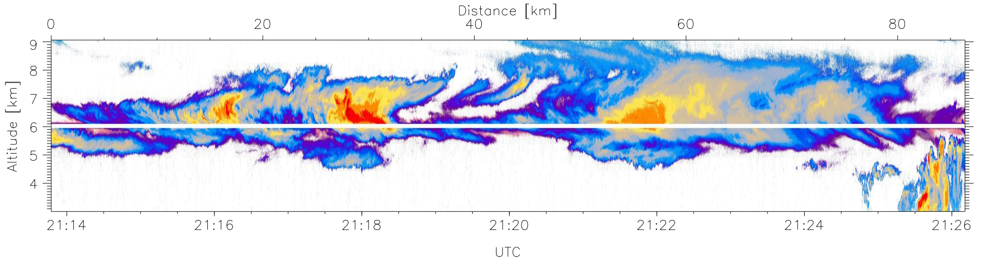
W2009-06-05-21-13-46, Up and Down Reflectivity
