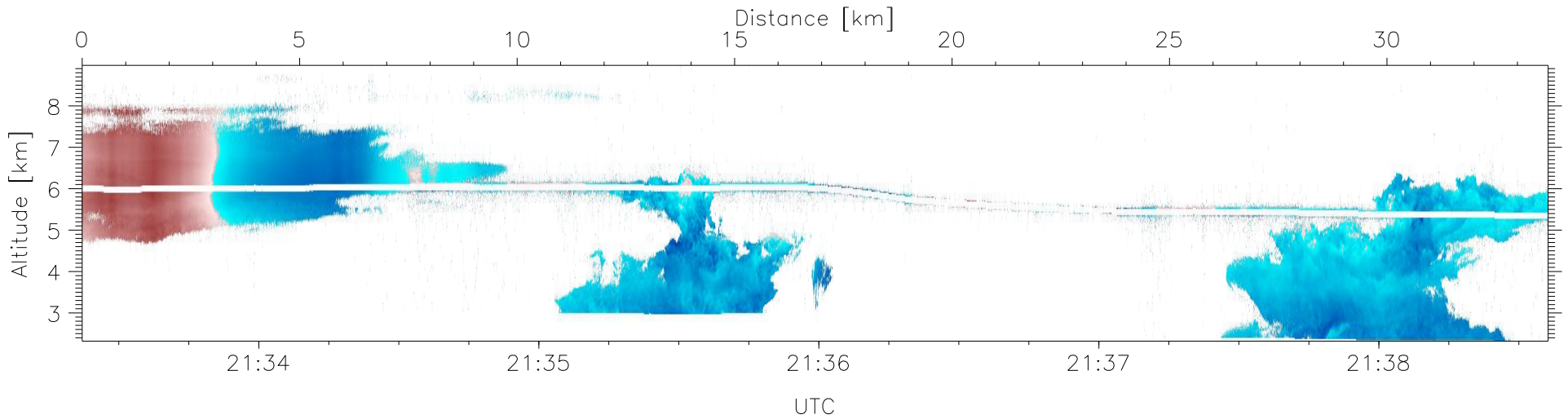
W2009-06-05-21-33-22, Up and Down Doppler
