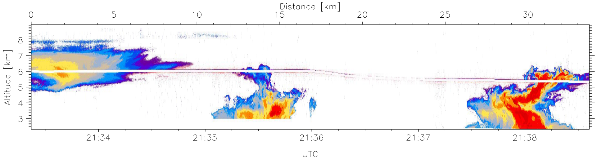
W2009-06-05-21-33-22, Up and Down Reflectivity
