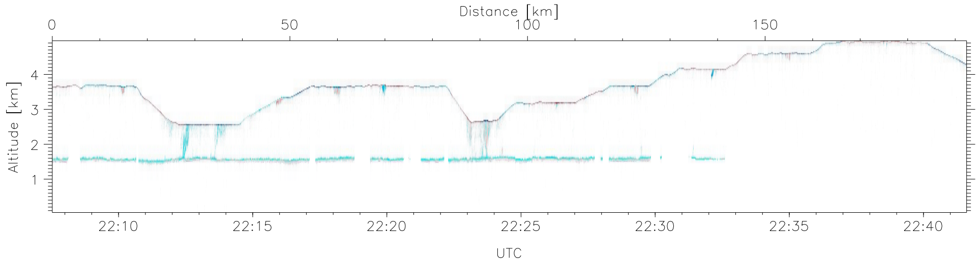
W2009-06-05-22-07-32: Down-slant Doppler
