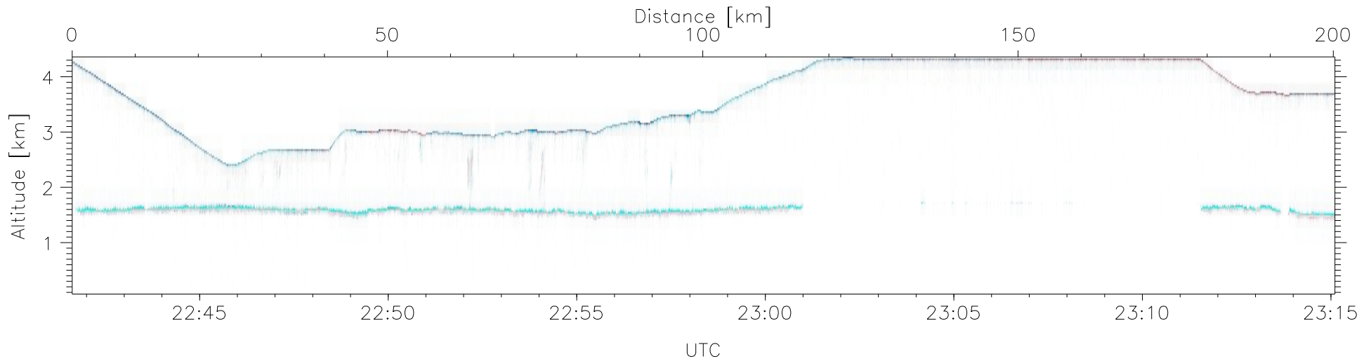
W2009-06-05-22-41-37: Down-slant Doppler
