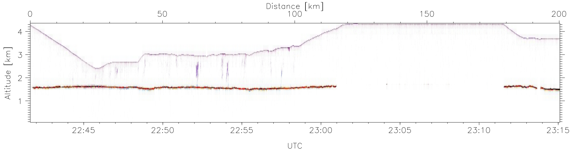
W2009-06-05-22-41-37: Down-slant Reflectivity
