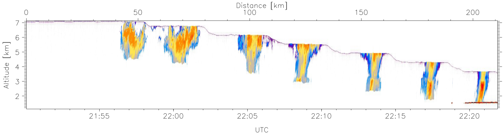
W2009-06-06-21-50-04: Down-slant Reflectivity
