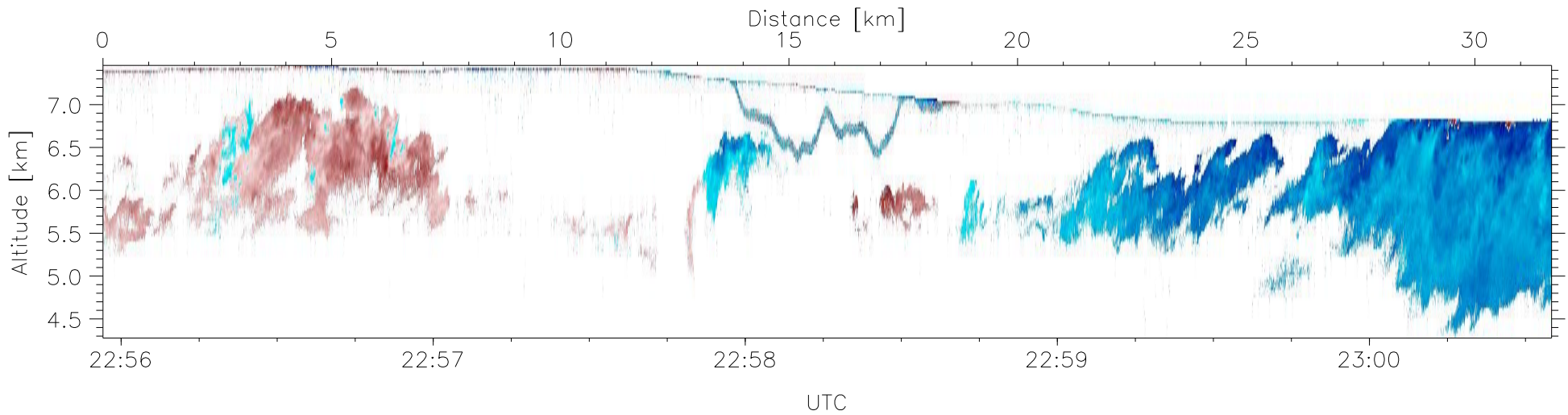
W2009-06-06-22-55-13: Down-slant Doppler
