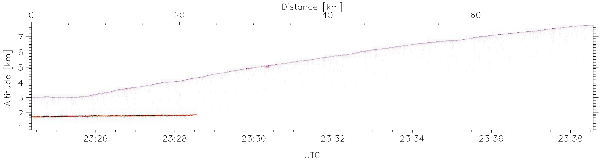
W2009-06-06-23-24-22: Down-slant Reflectivity
