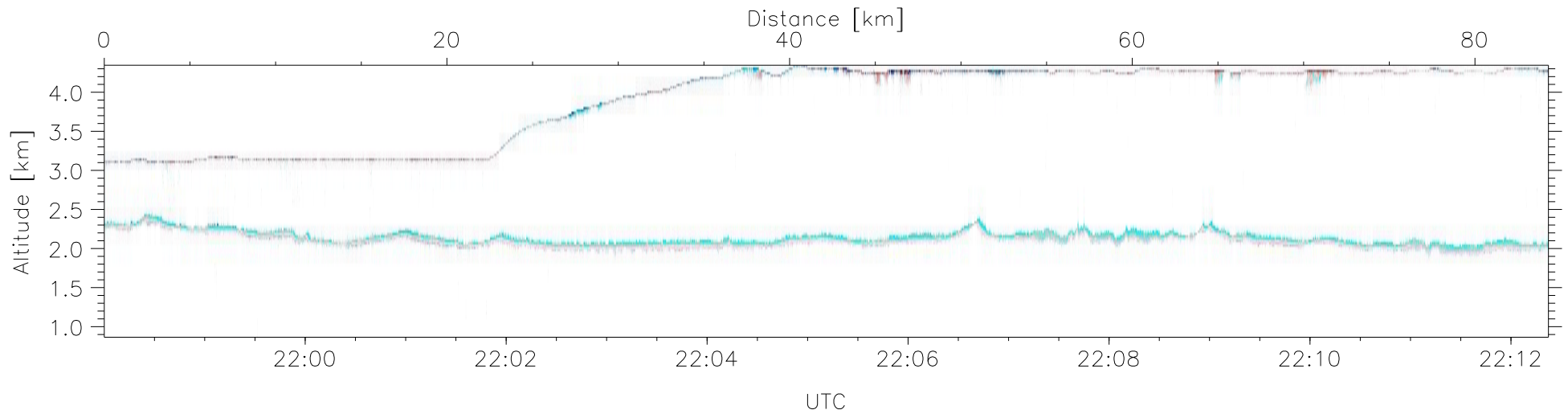
W2009-05-21-21-39-45: Down-slant Doppler
