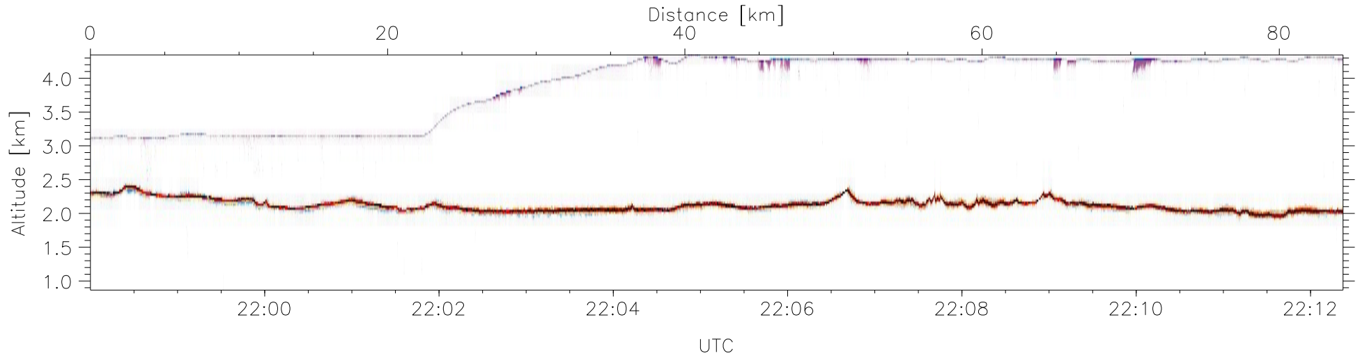
W2009-05-21-21-39-45: Down-slant Reflectivity
