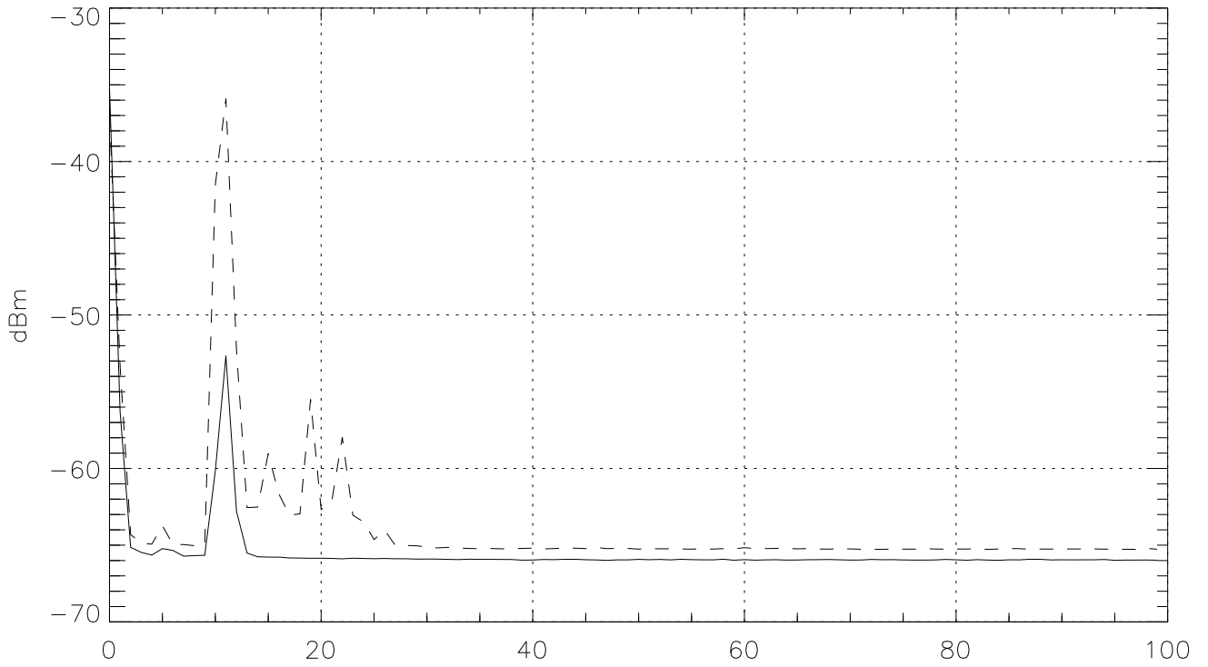
Wpp01-07-12-01-45-47 VV(42 deg aft) H antenna plugged, Signal from wide building leaks to V; vv -, hv --
