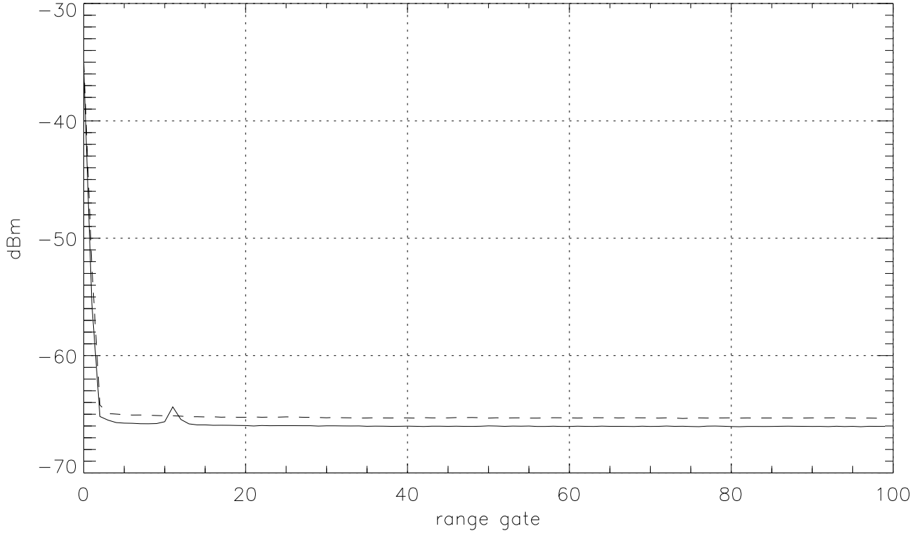
Wpp01-07-12-01-45-47 VV(42 deg aft) H antenna plugged, Signal from wide building leaks to V; vv -, hv --
