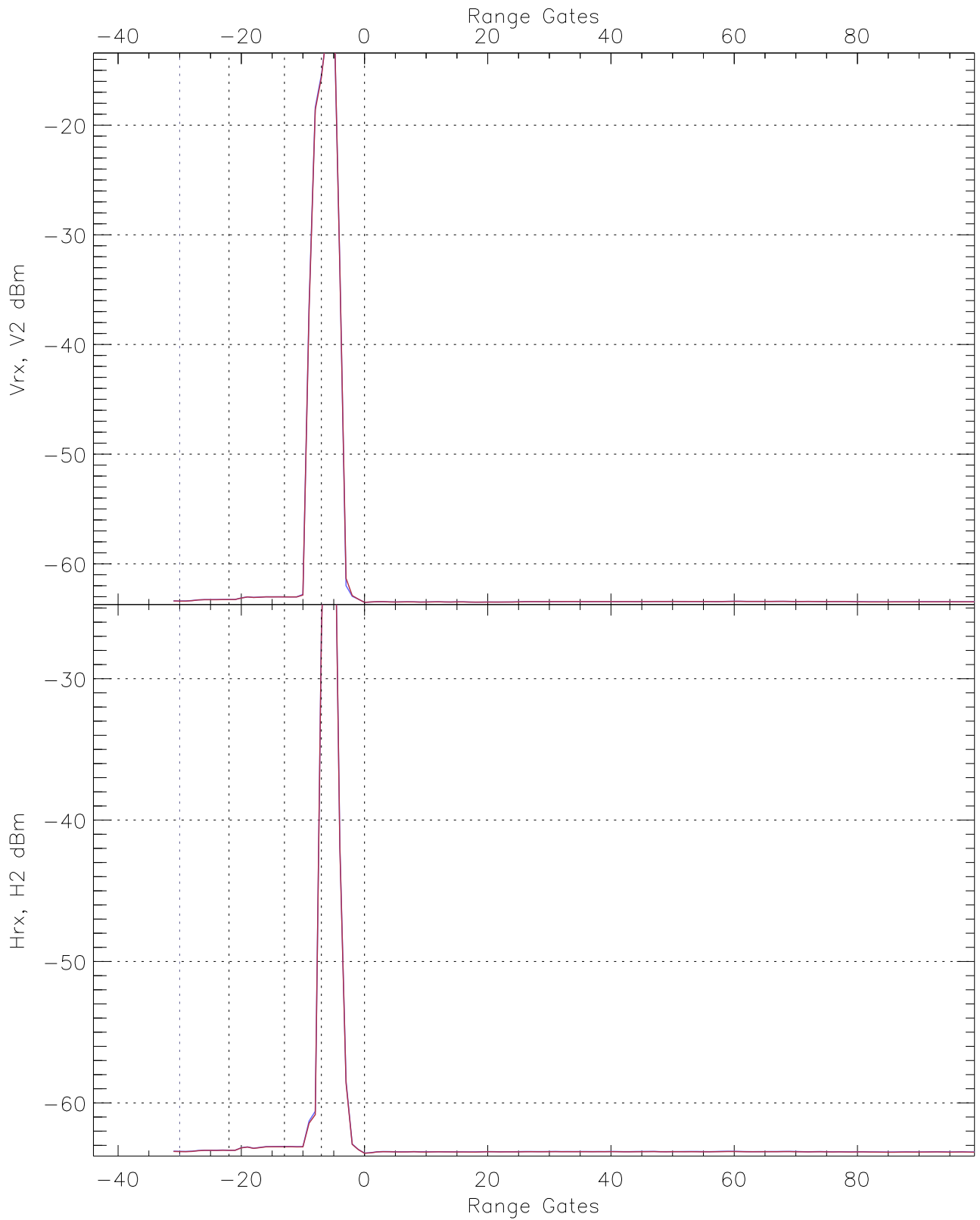
WCR2 CPP Averaged Received power for up 100 gates blue: 075032-075946, 12585 profiles averaged red: 075946-080900, 12584 profiles averaged
