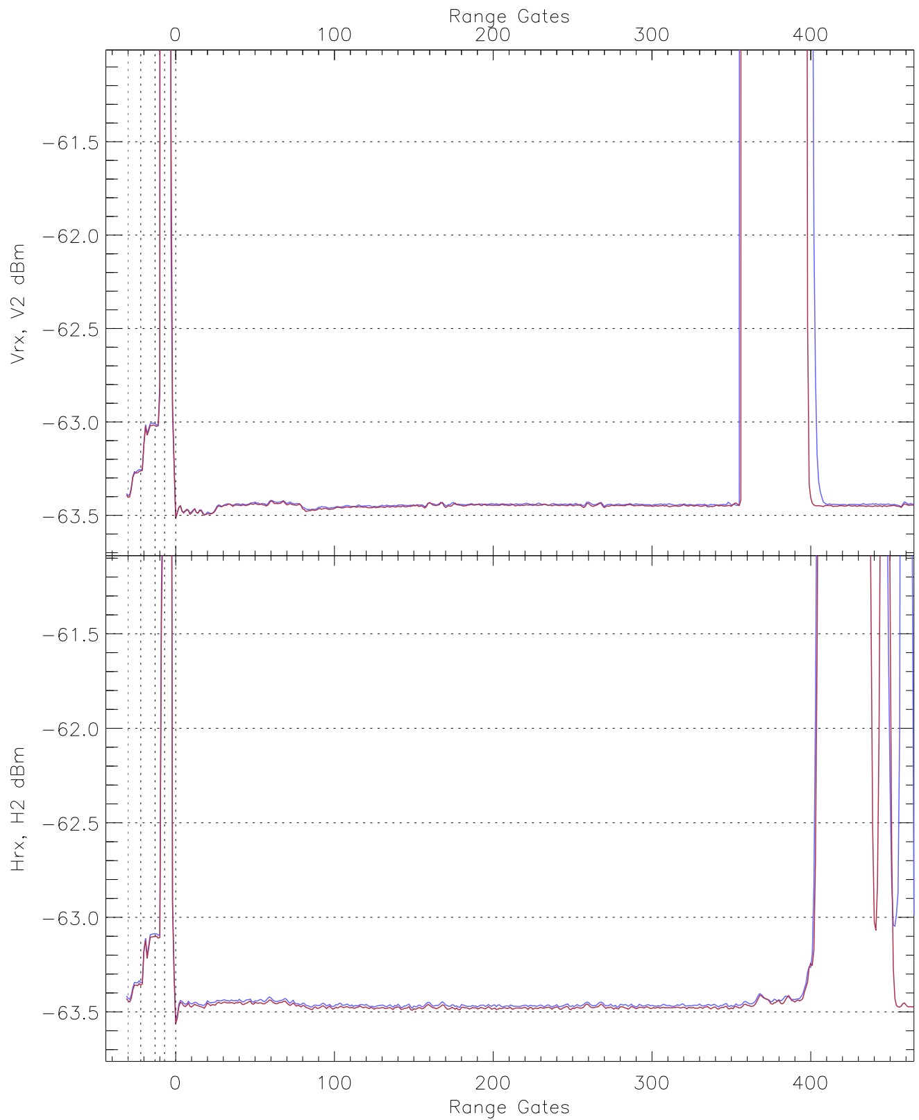
WCR2 CPP Averaged Received power for all recorded gates blue: 075032-075946, 12585 profiles averaged red: 075946-080900, 12584 profiles averaged
