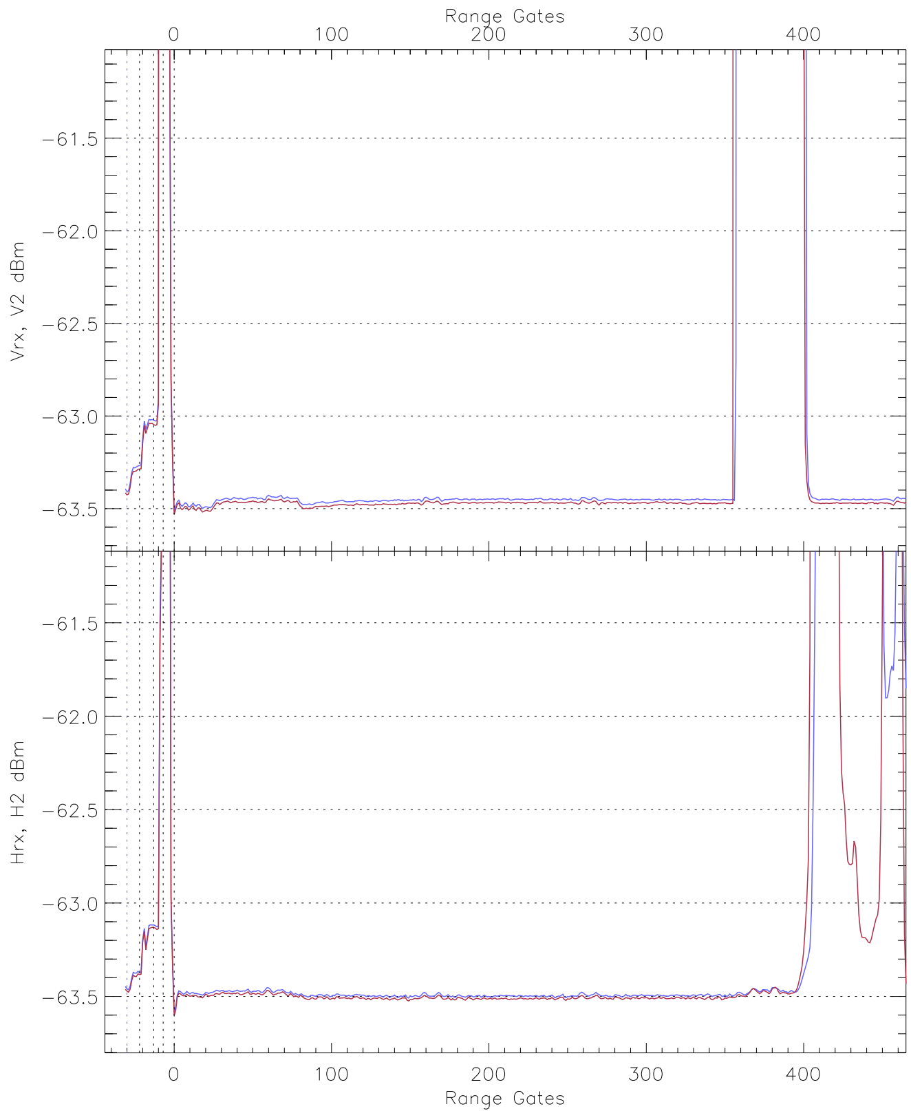
WCR2 CPP Averaged Received power for all recorded gates blue: 080902-082033, 15704 profiles averaged red: 082033-083204, 15704 profiles averaged
