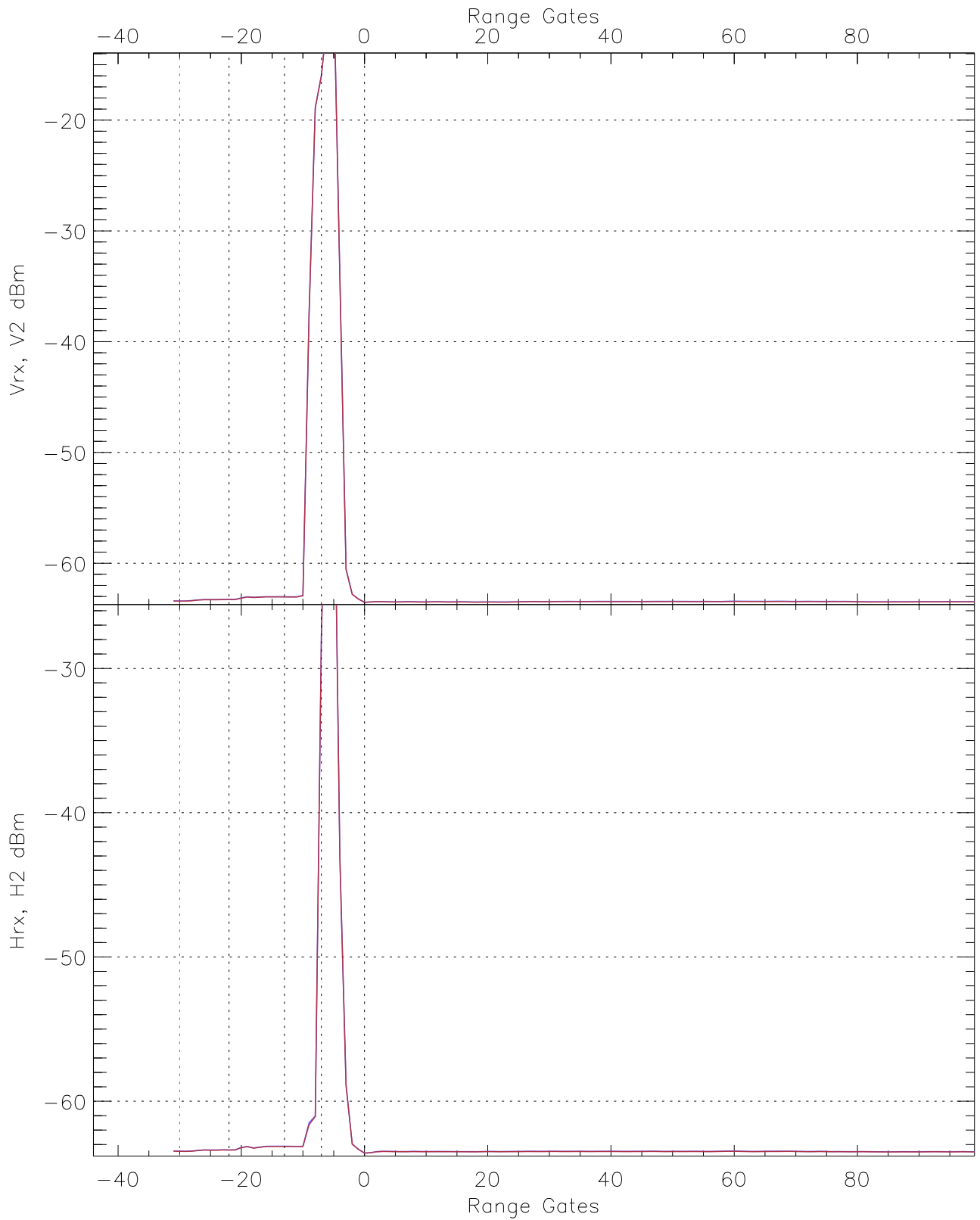
WCR2 CPP Averaged Received power for up 100 gates blue: 080902-082033, 15704 profiles averaged red: 082033-083204, 15704 profiles averaged
