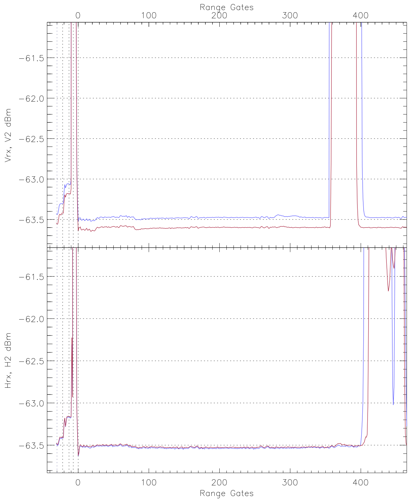
WCR2 CPP Averaged Received power for all recorded gates blue: 091301-092157, 12177 profiles averaged red: 092157-093053, 12177 profiles averaged
