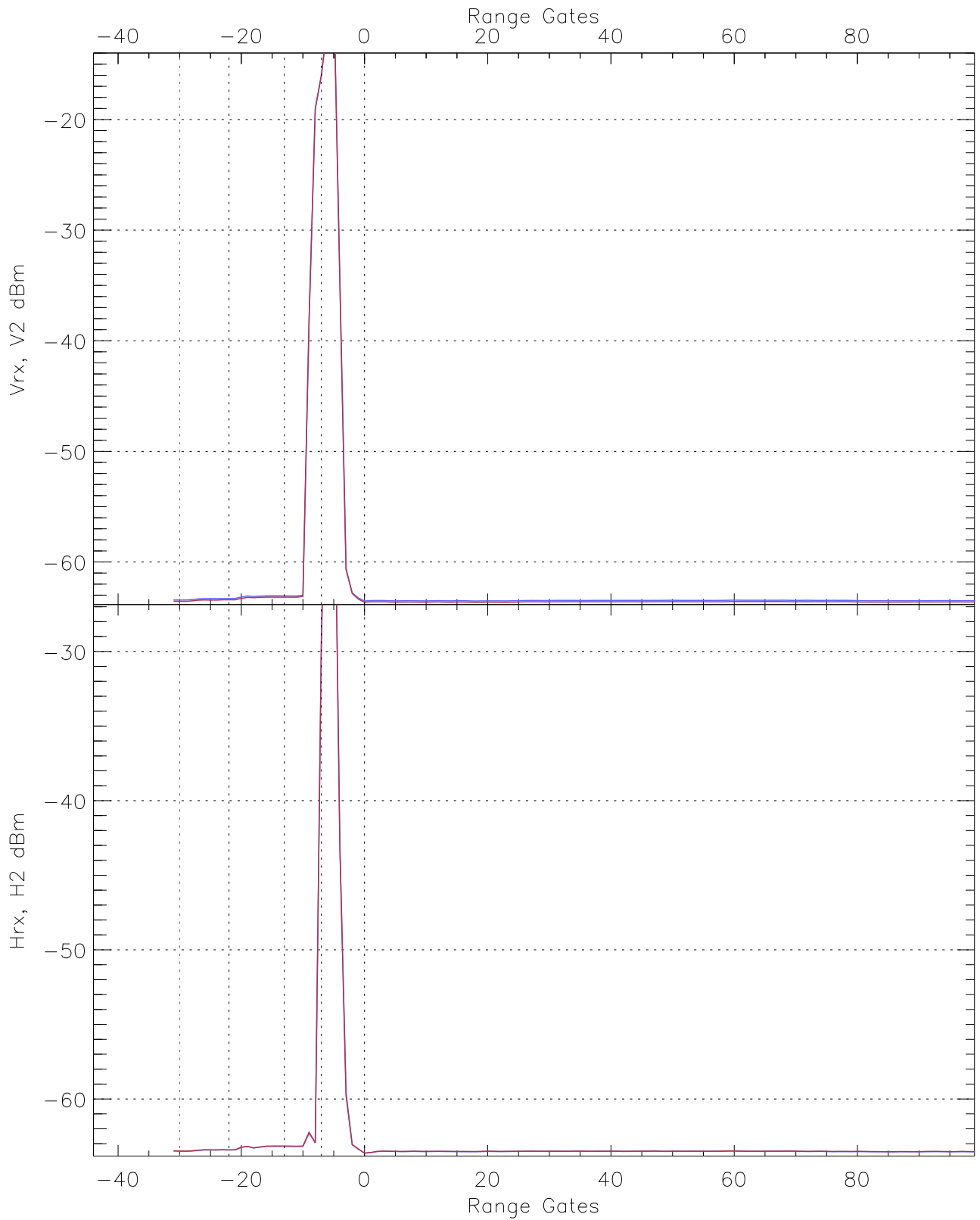
WCR2 CPP Averaged Received power for up 100 gates blue: 091301-092157, 12177 profiles averaged red: 092157-093053, 12177 profiles averaged
