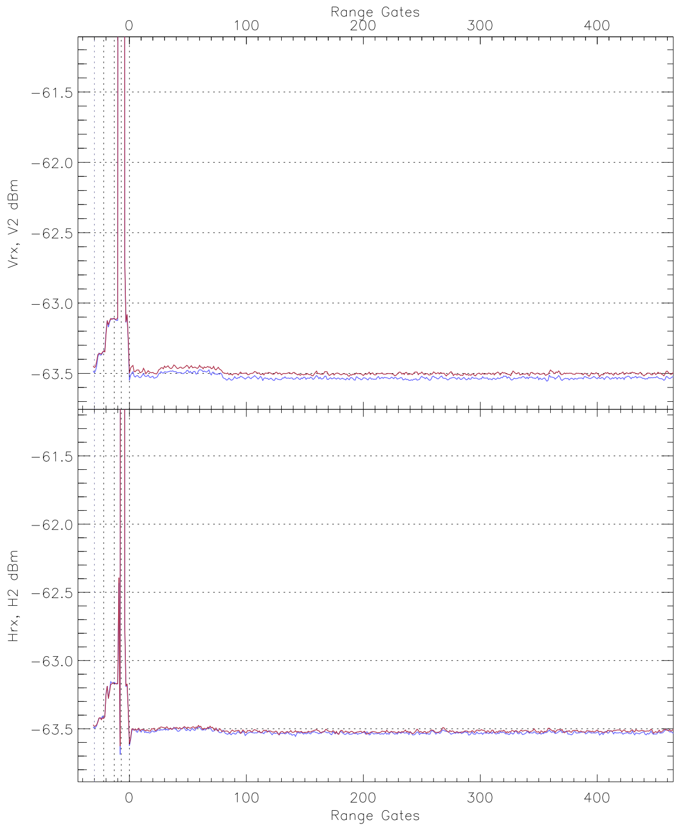
WCR2 CPP Averaged Received power for all recorded gates blue: 093216-093320, 1441 profiles averaged red: 093320-093423, 1441 profiles averaged
