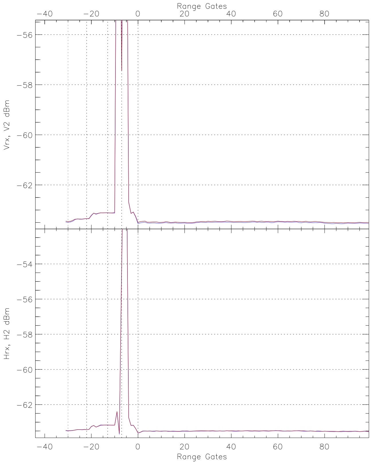
WCR2 CPP Averaged Received power for up 100 gates blue: 093216-093320, 1441 profiles averaged red: 093320-093423, 1441 profiles averaged
