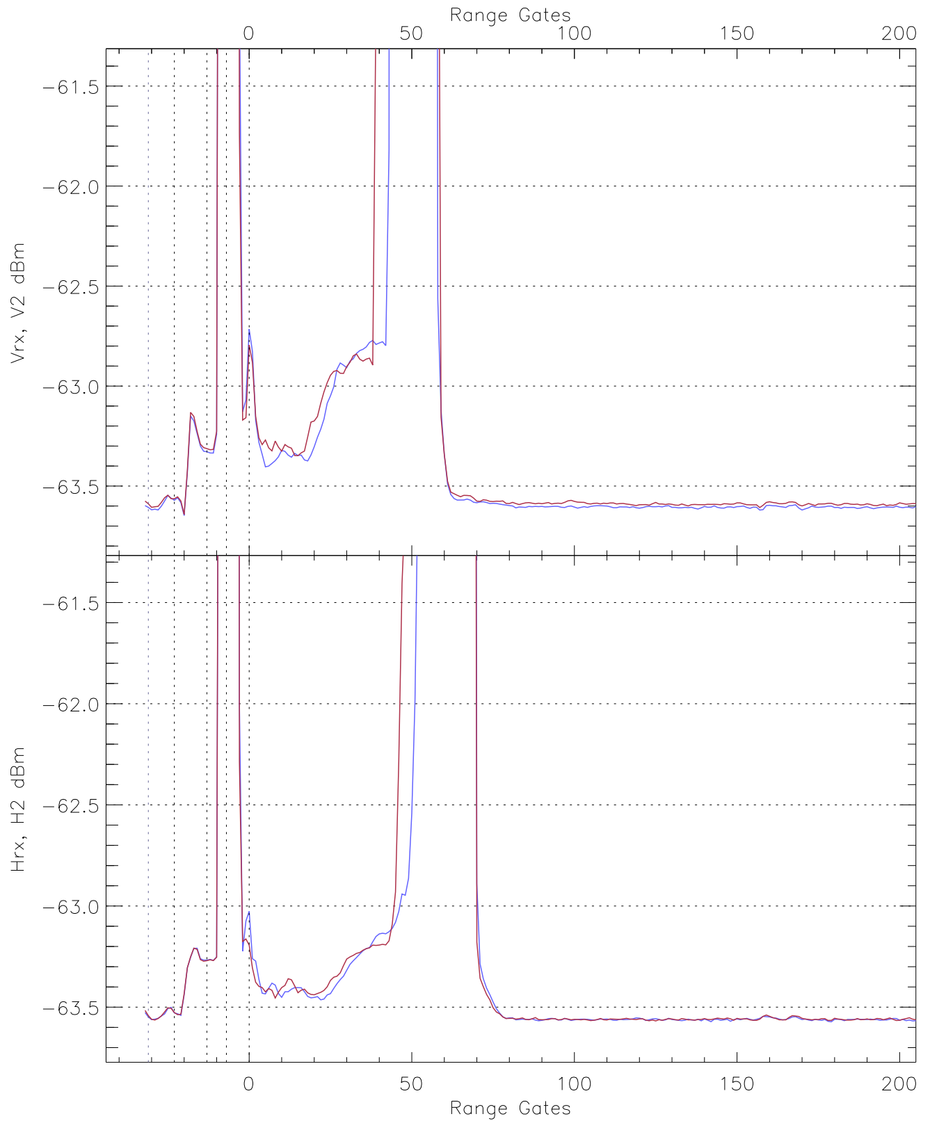
WCR2 CPP Averaged Received power for all recorded gates blue: 213509-213849, 5523 profiles averaged red: 213849-214231, 5522 profiles averaged
