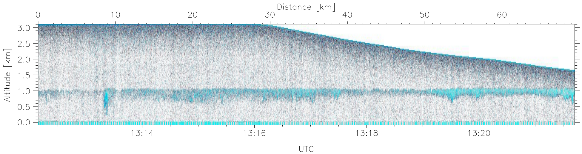
W2008-11-15-13-12-08: Down Doppler
