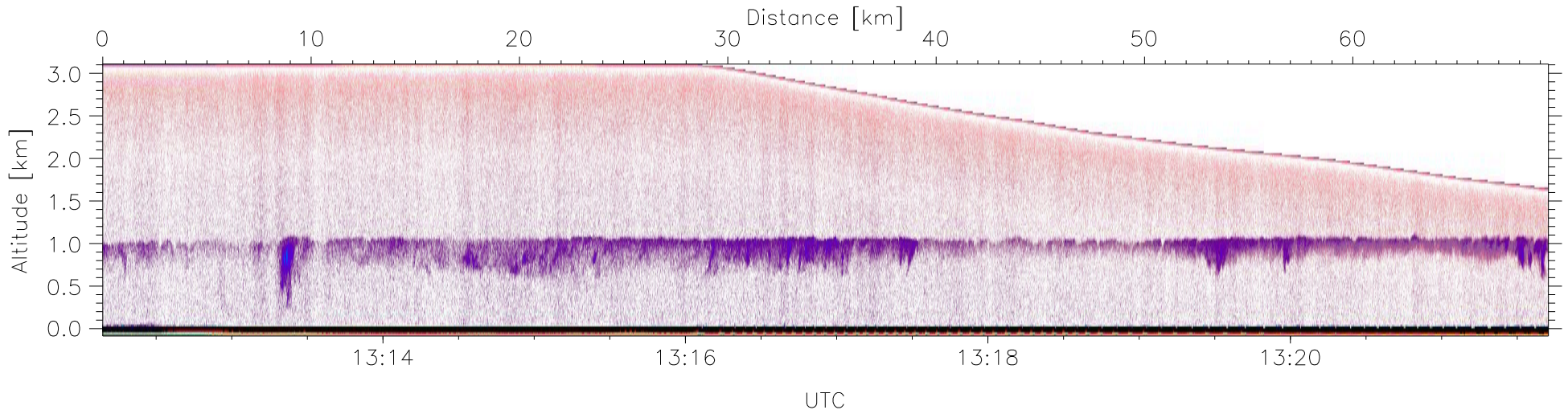
W2008-11-15-13-12-08: Down Reflectivity
