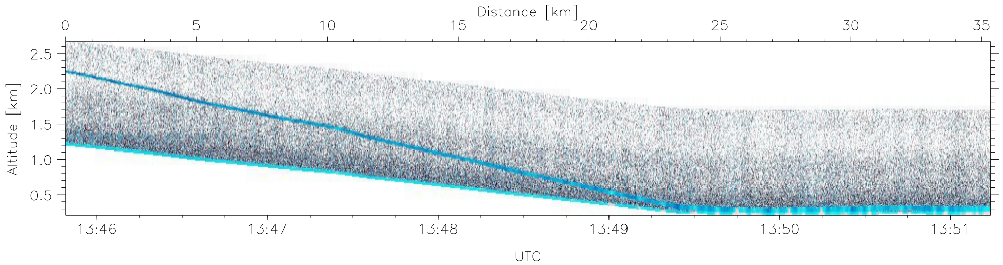
W2008-11-15-13-45-48: Up Doppler
