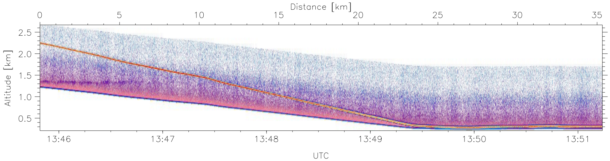
W2008-11-15-13-45-48: Up Reflectivity
