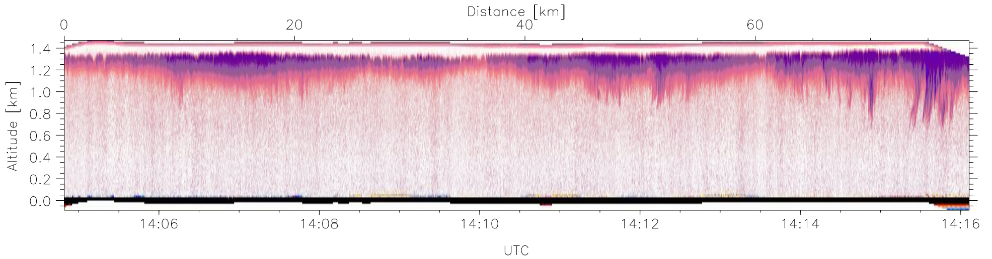
W2008-11-15-14-04-48: Down Reflectivity
