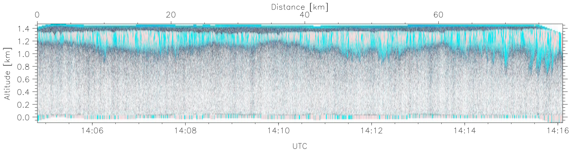
W2008-11-15-14-04-48: Down Doppler
