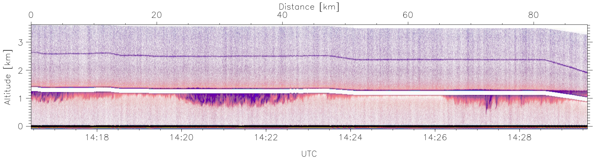
W2008-11-15-14-16-26, Up and Down Reflectivity
