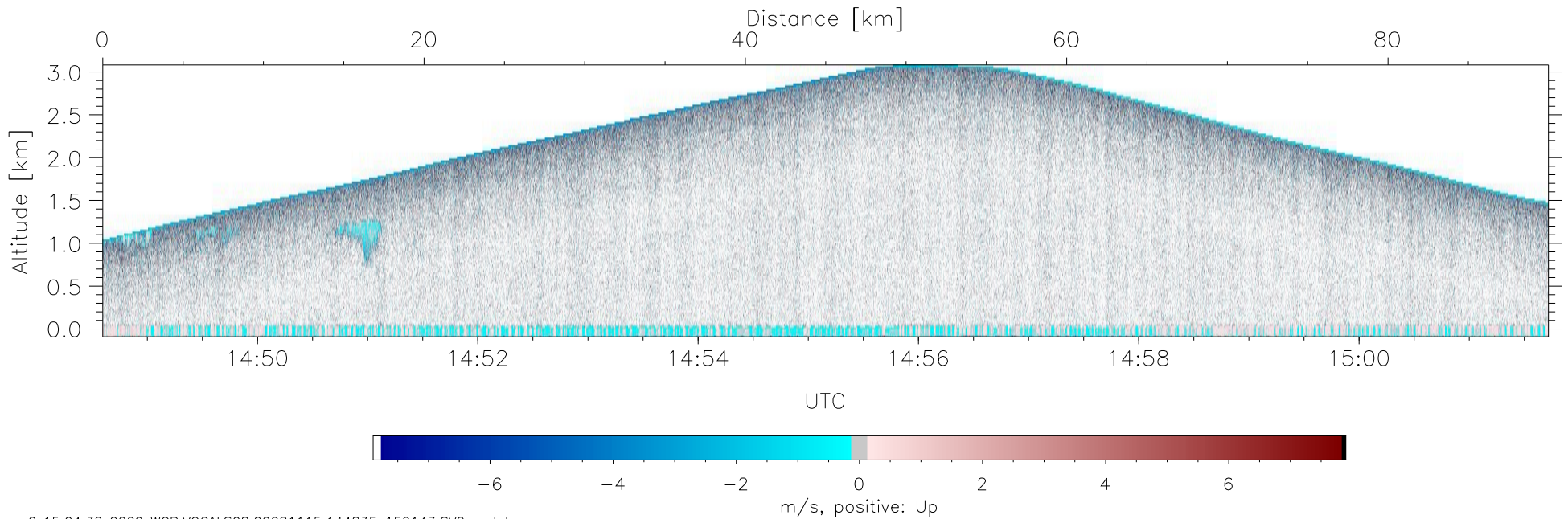
W2008-11-15-14-48-35: Down Doppler
