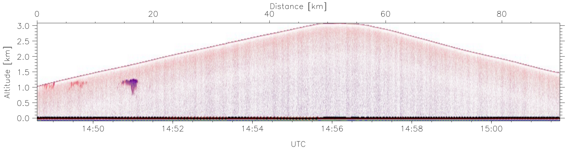
W2008-11-15-14-48-35: Down Reflectivity
