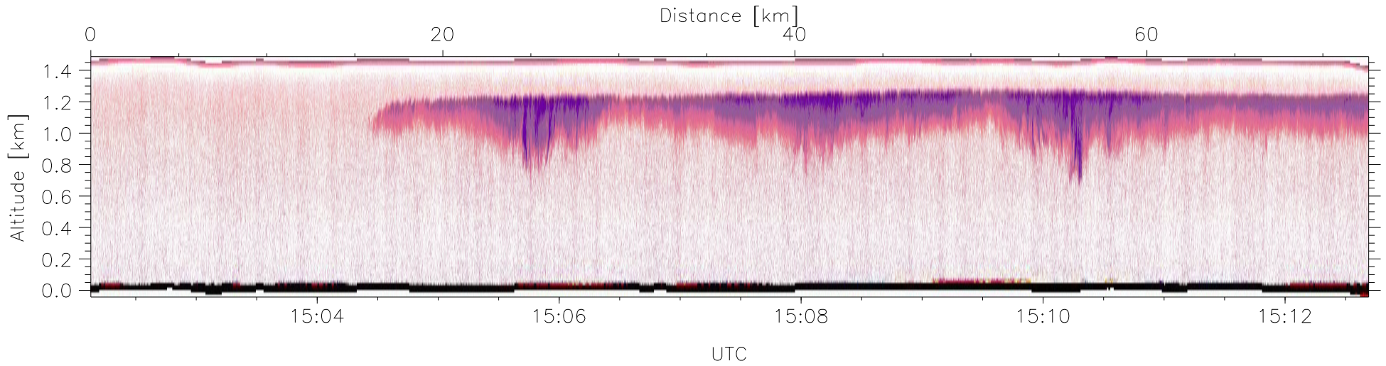
W2008-11-15-15-02-07: Down Reflectivity
