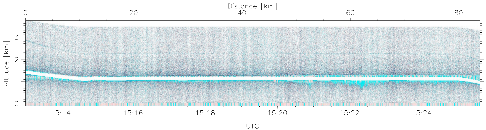
W2008-11-15-15-13-00, Up and Down Doppler
