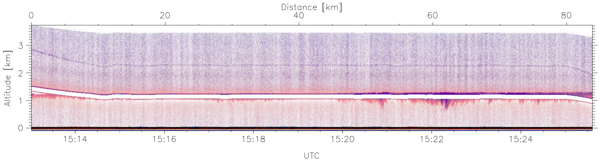
W2008-11-15-15-13-00, Up and Down Reflectivity
