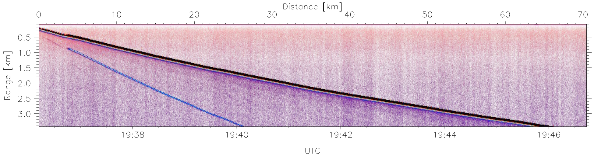
W2008-11-15-19-36-11: Down Reflectivity
