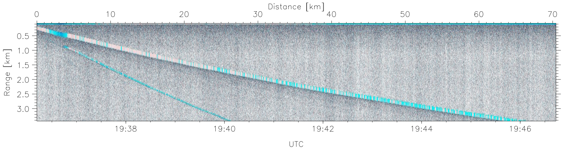
W2008-11-15-19-36-11: Down Doppler
