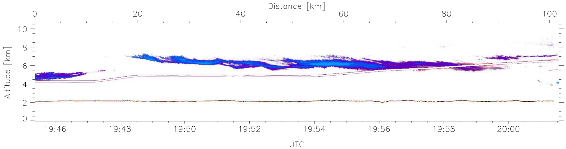
W2009-04-02-19-45-22, Up and Down Reflectivity
