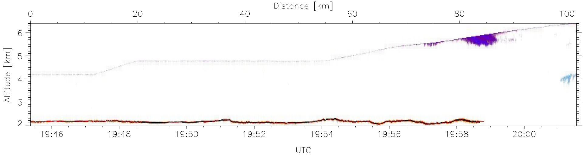
W2009-04-02-19-45-22: Down-slant Reflectivity
