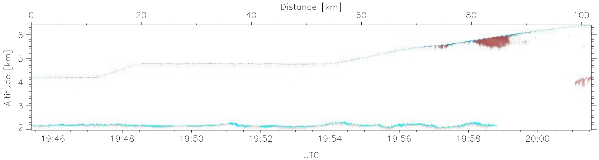
W2009-04-02-19-45-22: Down-slant Doppler
