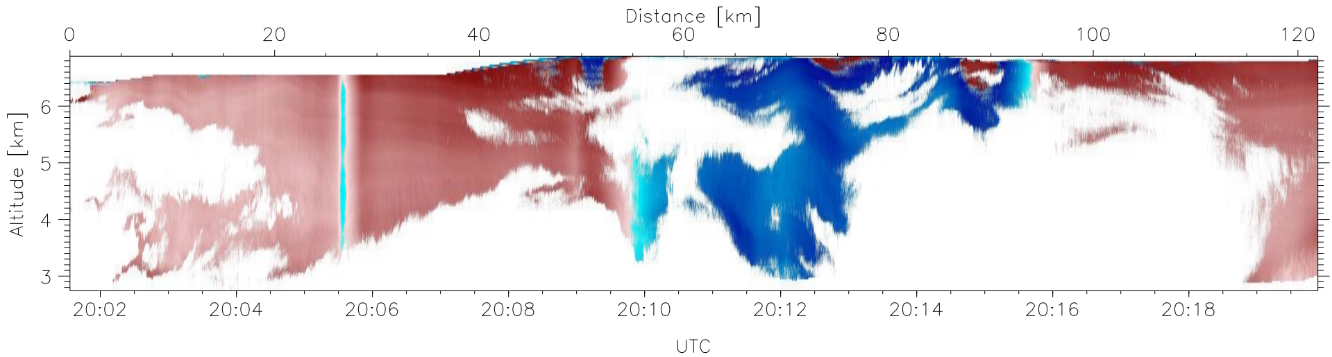
T2009-04-02-20-01-33: Down-slant Doppler
