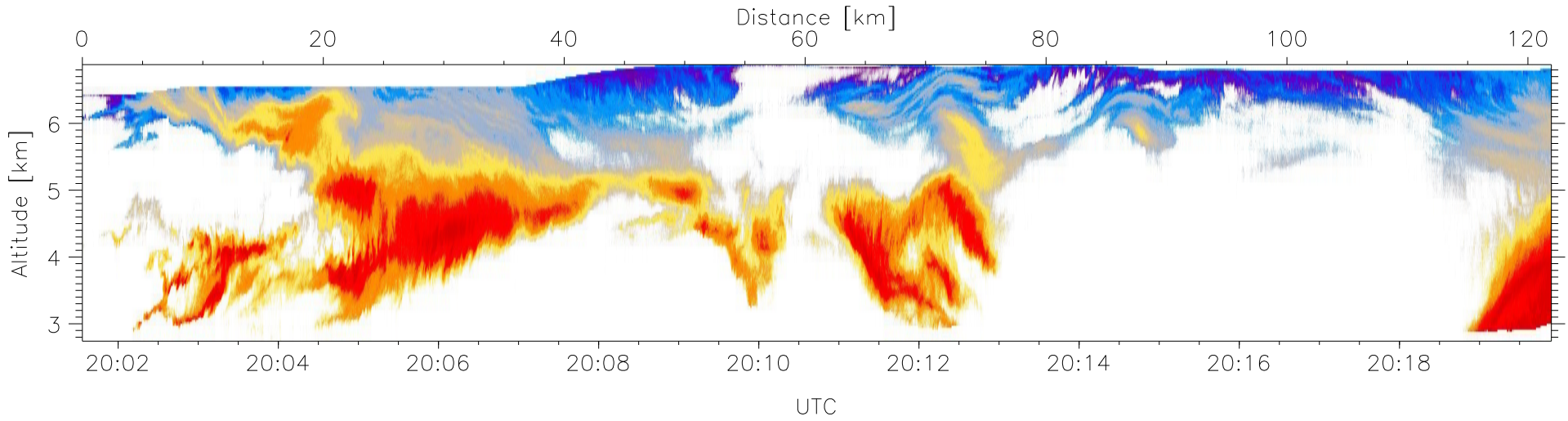
T2009-04-02-20-01-33: Down-slant Reflectivity
