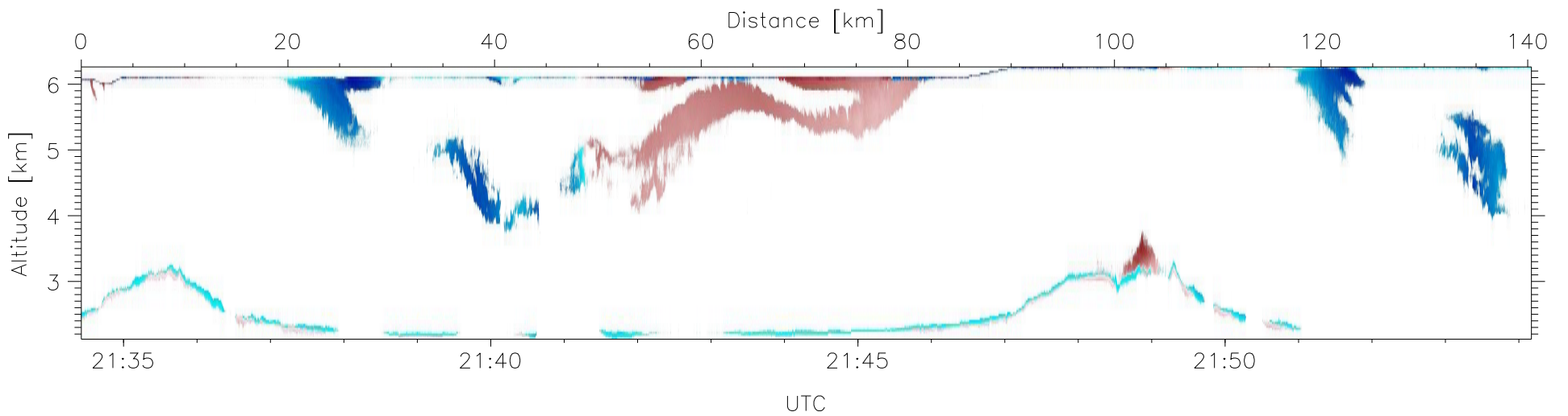
T2009-04-02-21-34-25: Down-slant Doppler
