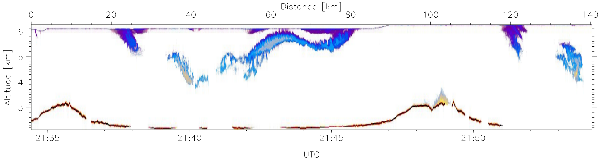
T2009-04-02-21-34-25: Down-slant Reflectivity
