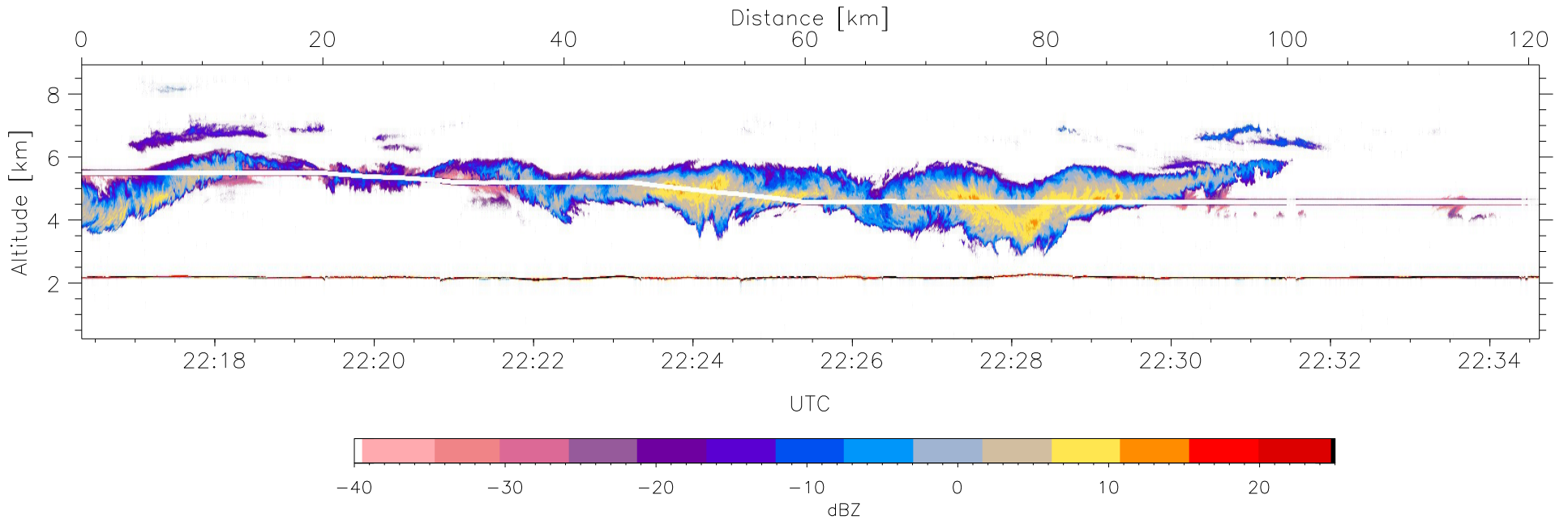
W2009-04-02-22-16-19, Up and Down Doppler, MaxVel Top/Bottom: 15.80/15.80
