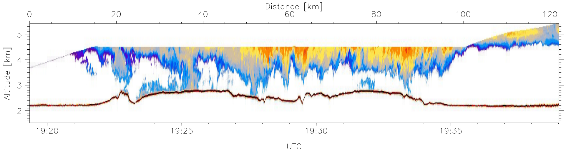
W2009-04-03-19-19-21: Down-slant Reflectivity
