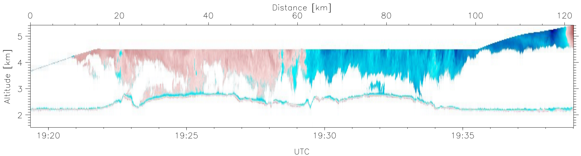
W2009-04-03-19-19-21: Down-slant Doppler
