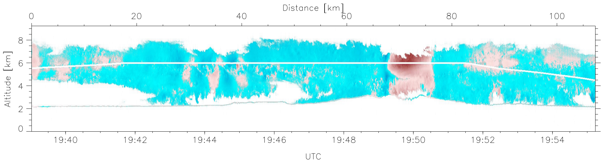
W2009-04-03-19-39-01, Up and Down Doppler, MaxVel Top/Bottom: 15.80/15.80
