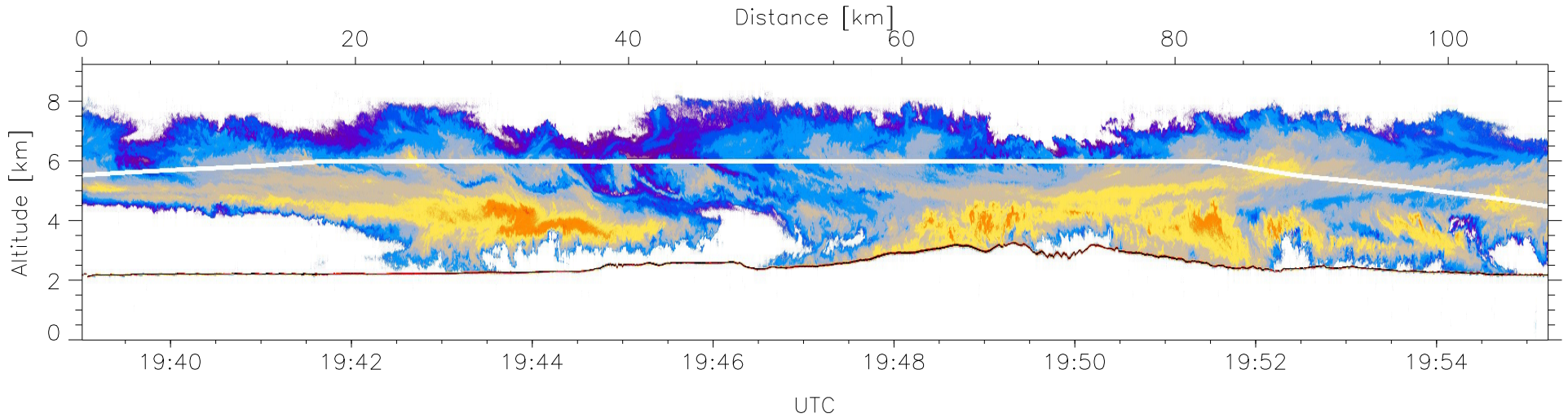
W2009-04-03-19-39-01, Up and Down Reflectivity
