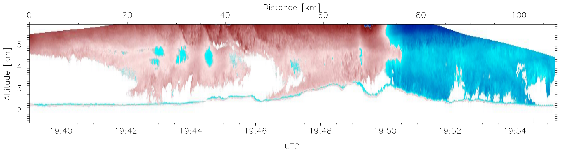
W2009-04-03-19-39-01: Down-slant Doppler
