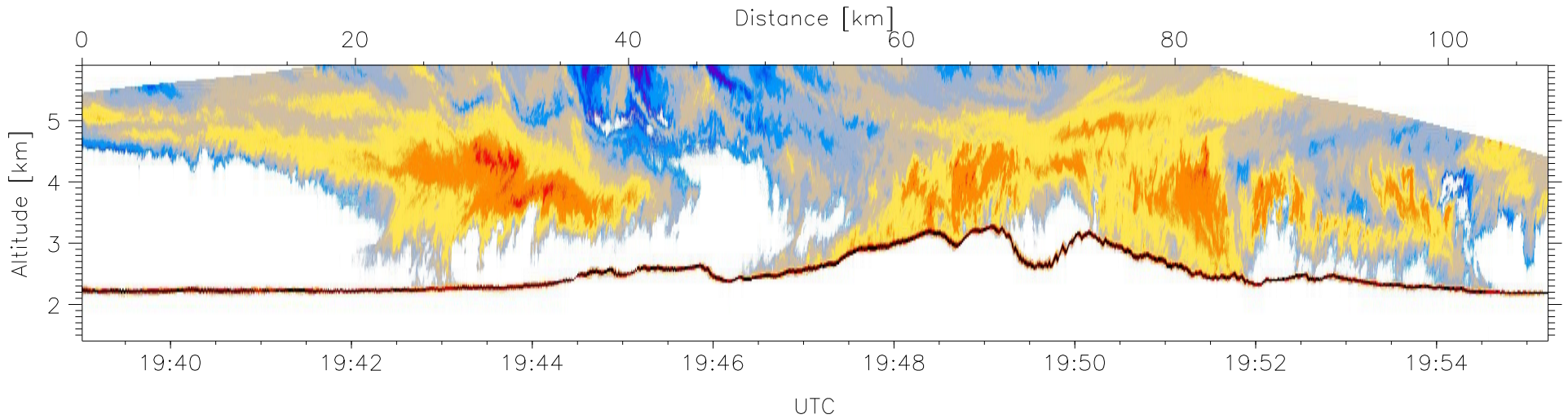
W2009-04-03-19-39-01: Down-slant Reflectivity
