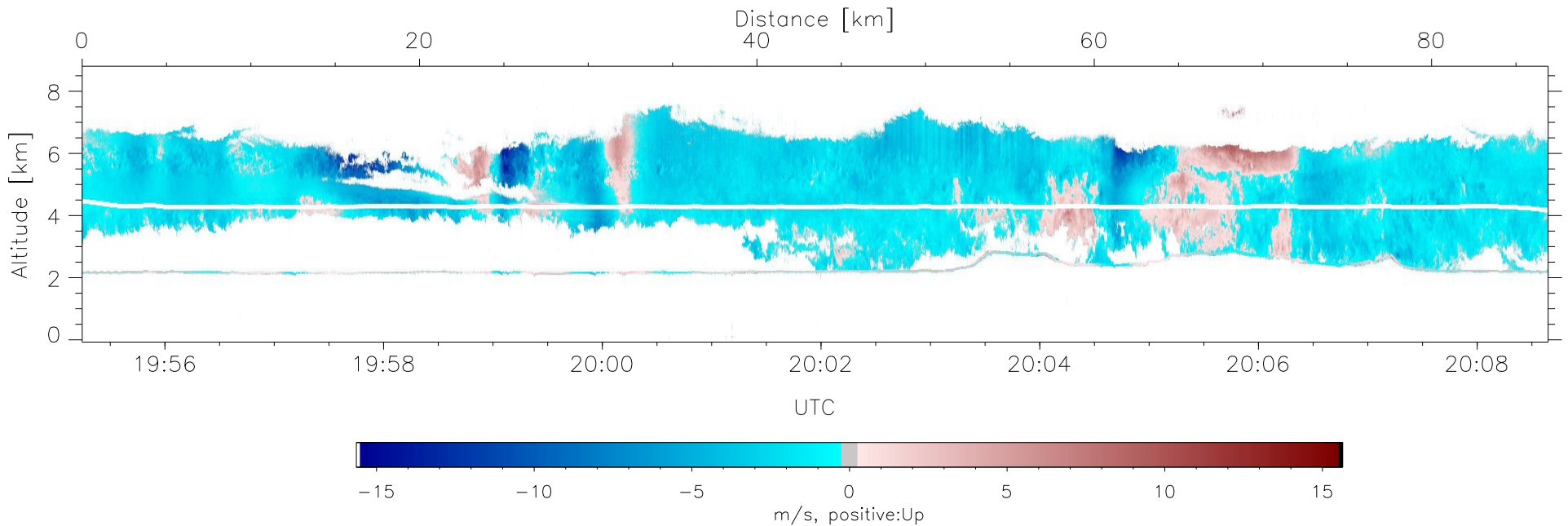
W2009-04-03-19-55-14, Up and Down Doppler, MaxVel Top/Bottom: 15.80/15.80
