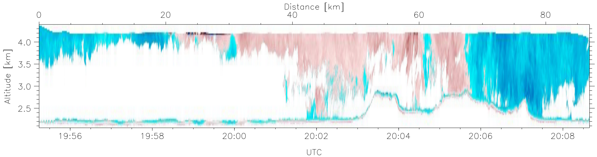
W2009-04-03-19-55-14: Down-slant Doppler
