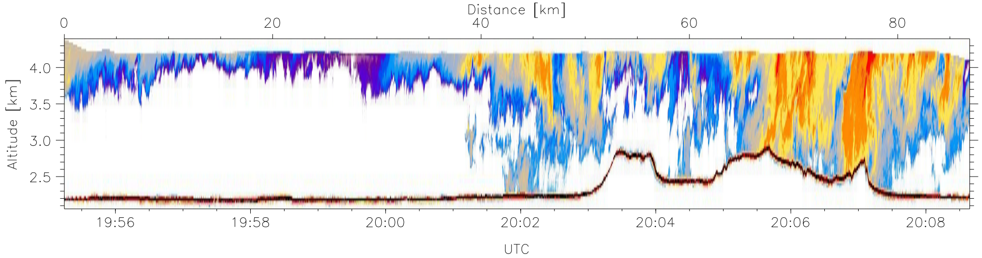
W2009-04-03-19-55-14: Down-slant Reflectivity
