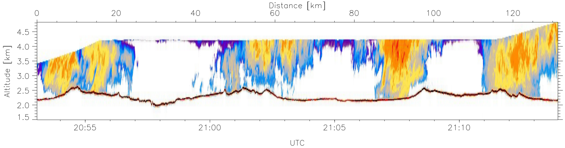
W2009-04-03-20-53-04: Down-slant Reflectivity
