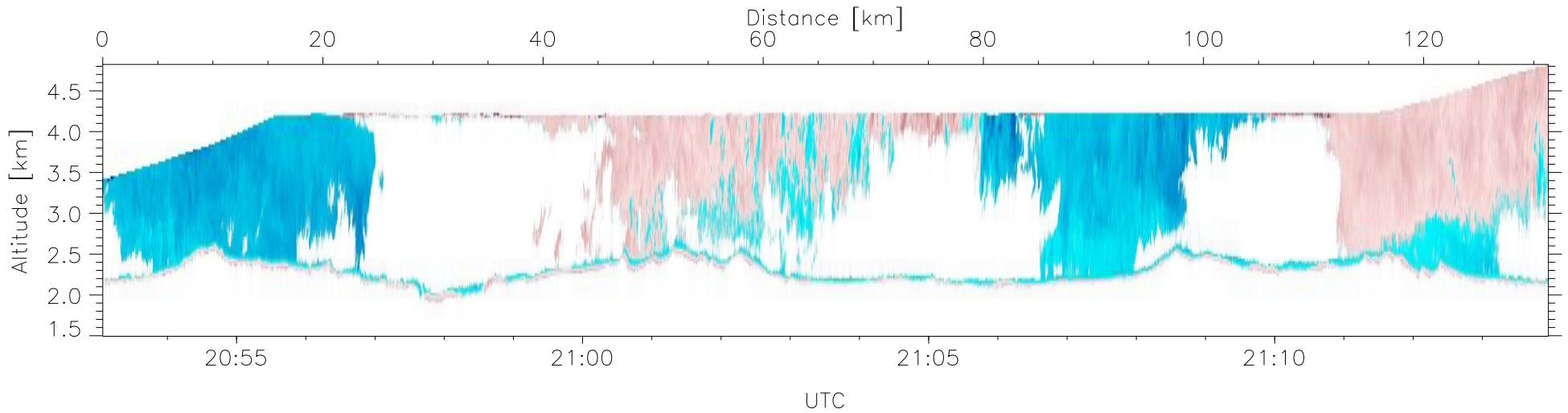
W2009-04-03-20-53-04: Down-slant Doppler
