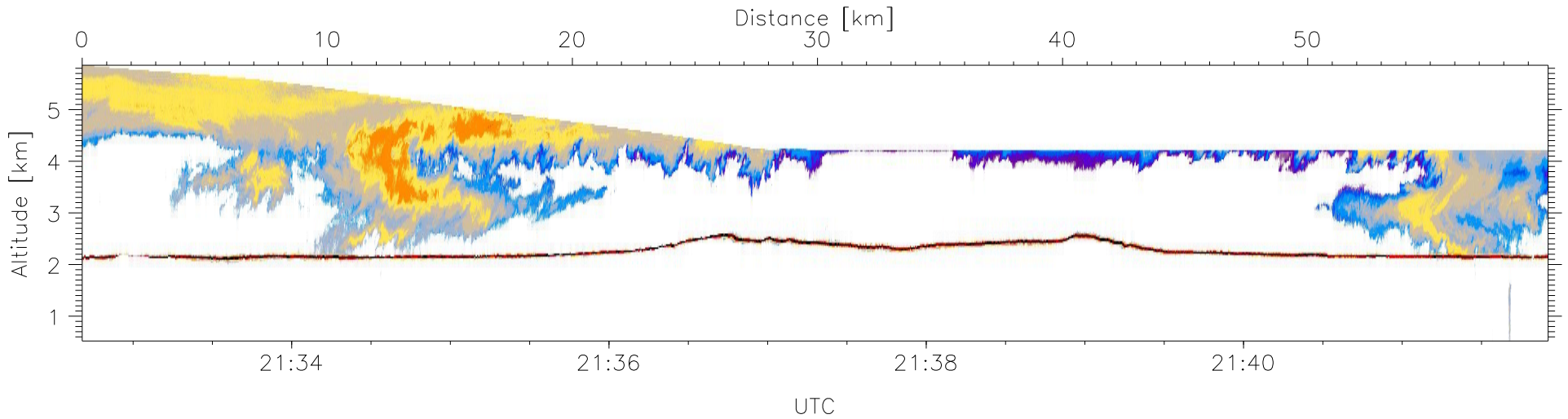
W2009-04-03-21-32-40: Down-slant Reflectivity
