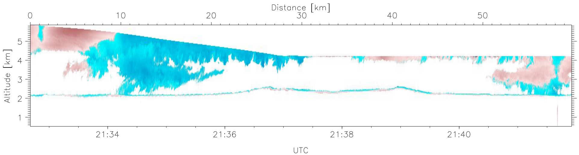
W2009-04-03-21-32-40: Down-slant Doppler
