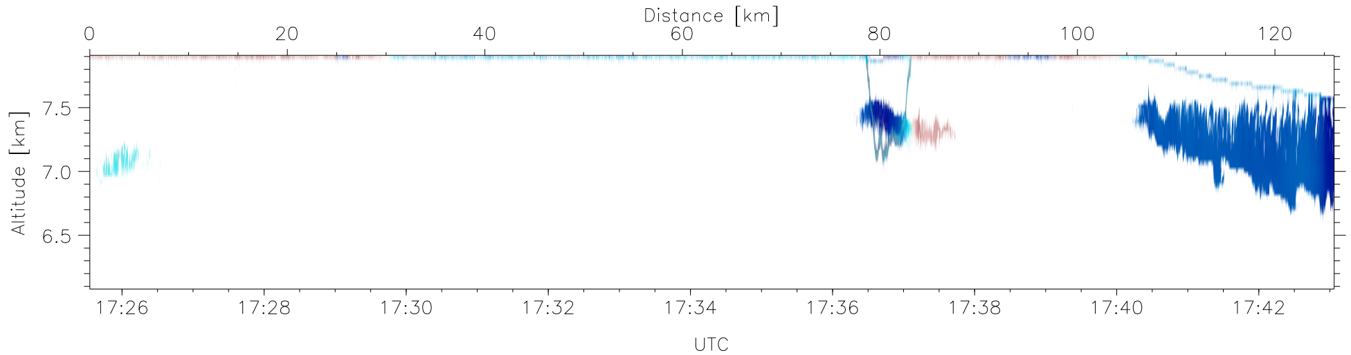
W2009-04-08-17-25-33: Down-slant Doppler
