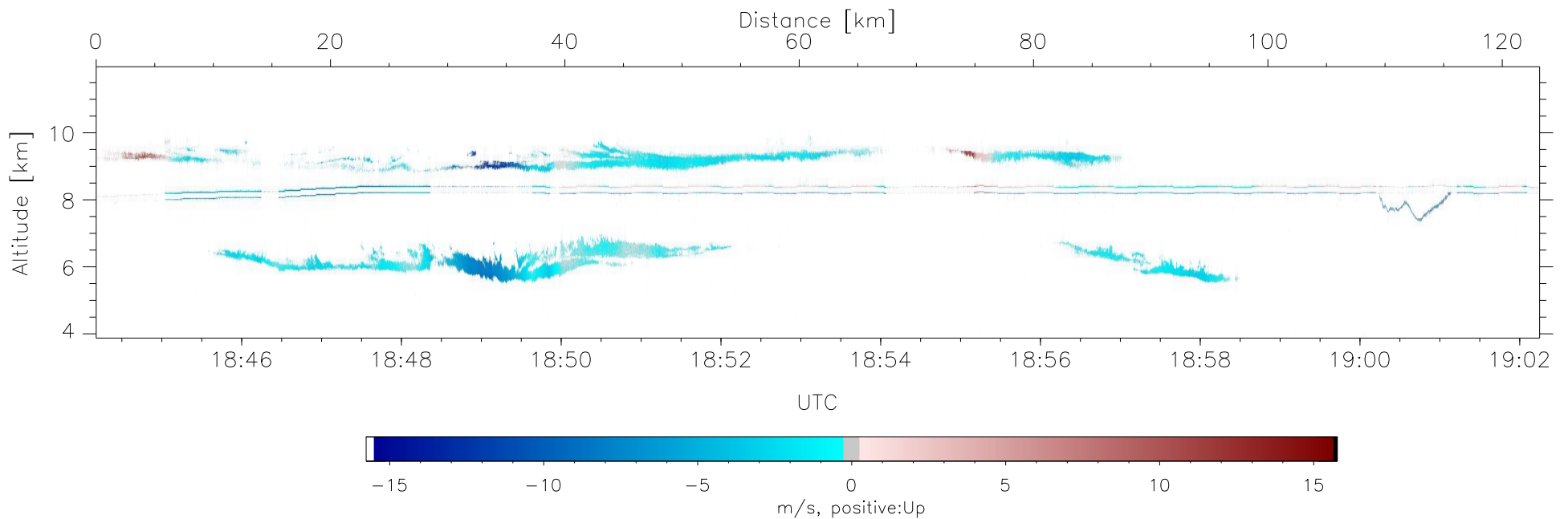
W2009-04-08-18-44-10, Up and Down Doppler, MaxVel Top/Bottom: 15.80/15.80
