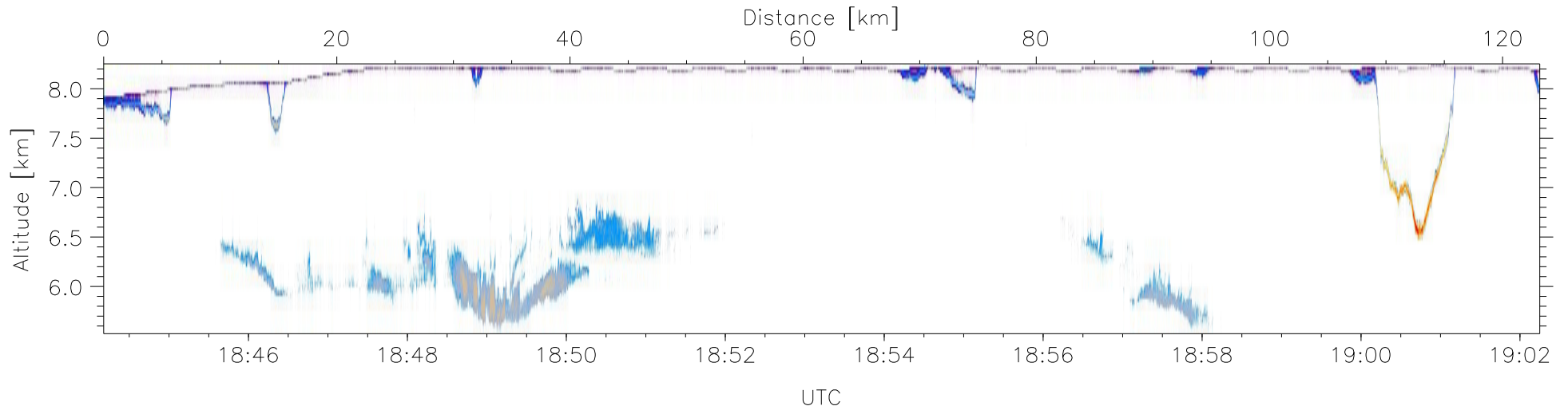
W2009-04-08-18-44-10: Down-slant Reflectivity
