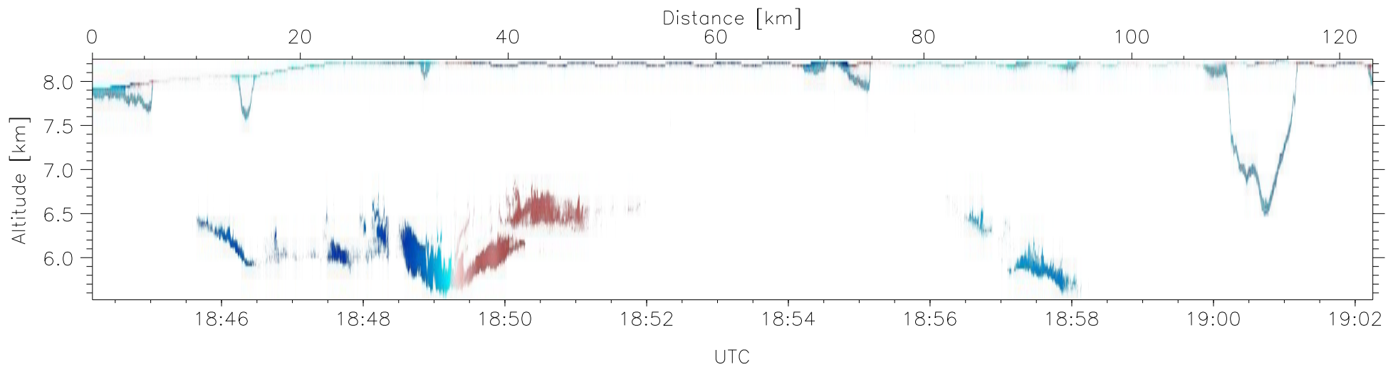
W2009-04-08-18-44-10: Down-slant Doppler
