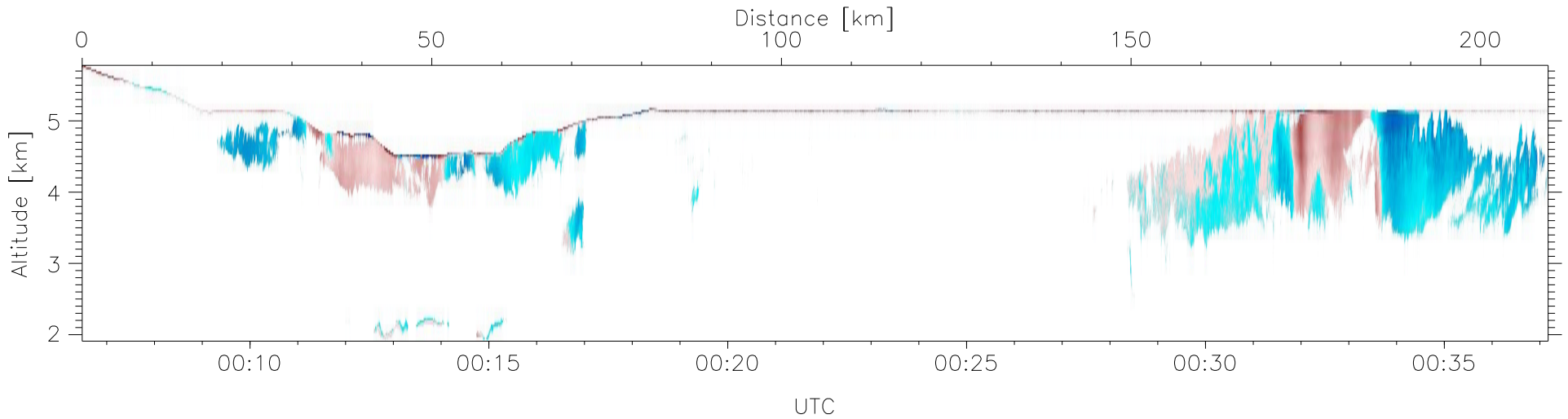
W2009-04-11-00-06-29: Down-slant Doppler
