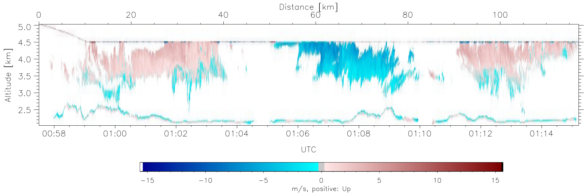
W2009-04-11-00-37-10: Down-slant Doppler
