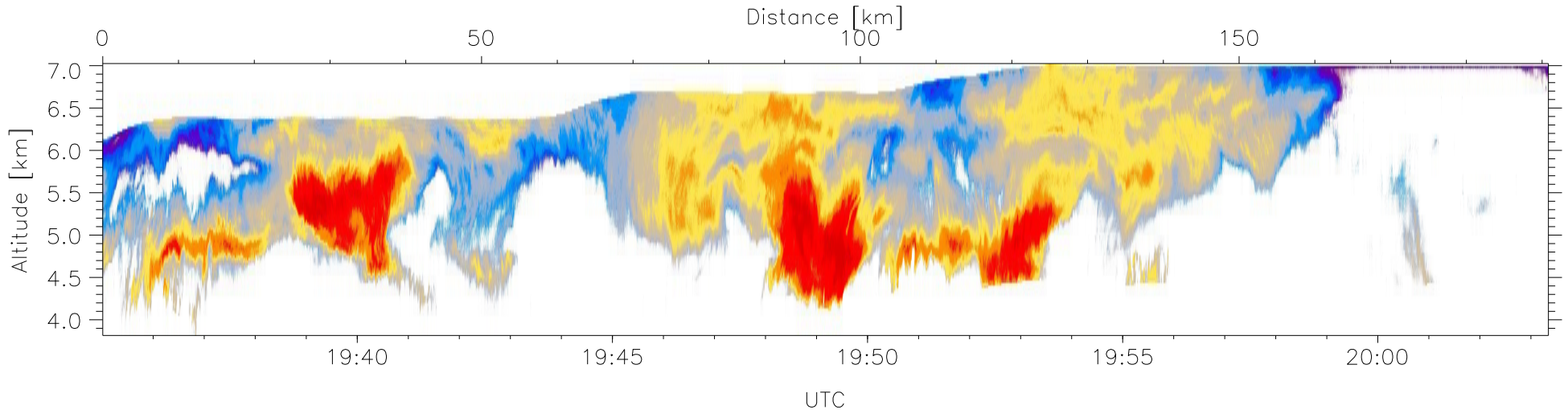
W2009-04-14-19-35-00: Down-slant Reflectivity
