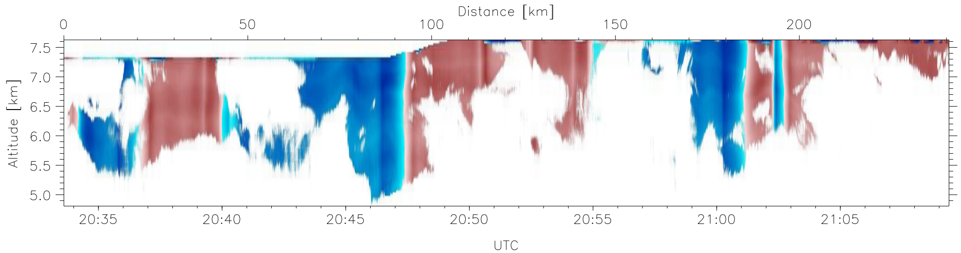
W2009-04-14-20-33-36: Down-slant Doppler
