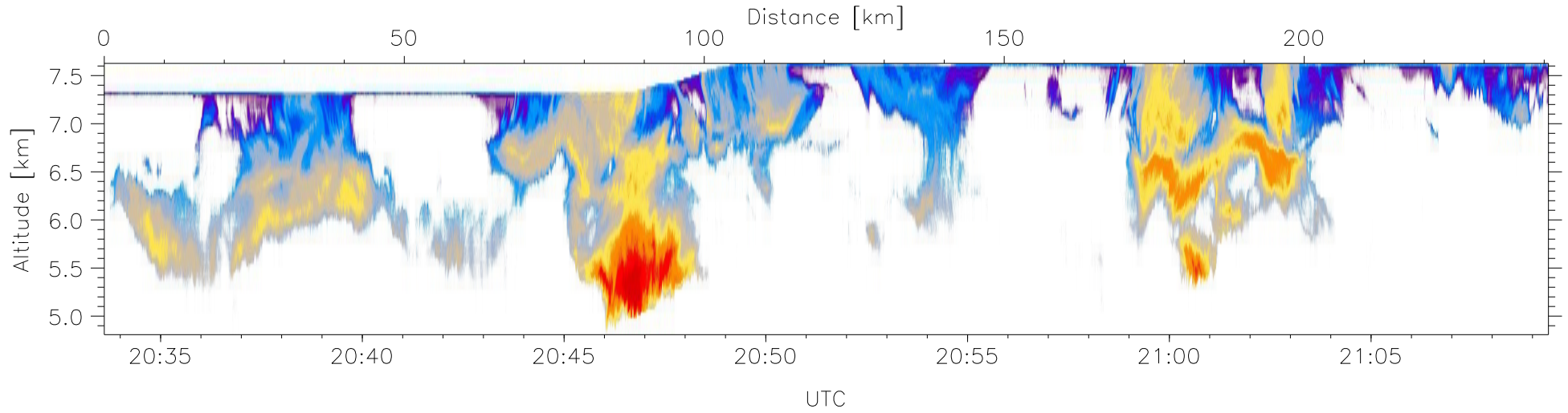
W2009-04-14-20-33-36: Down-slant Reflectivity
