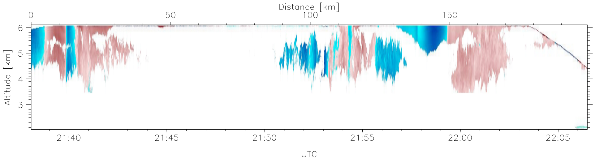
W2009-04-14-21-38-04: Down-slant Doppler
