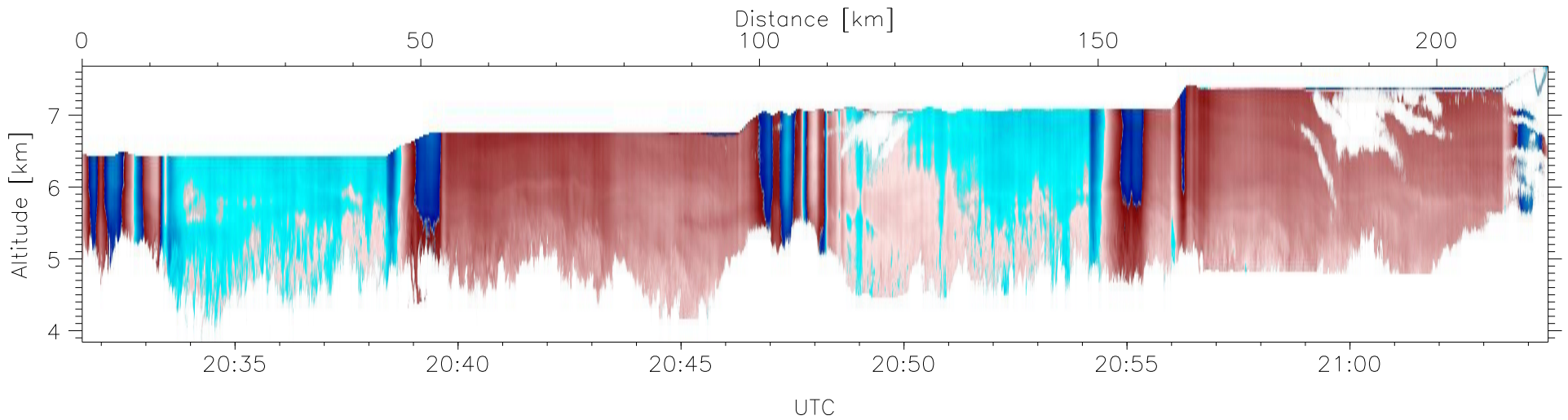
W2009-04-30-20-31-34: Down-slant Doppler
