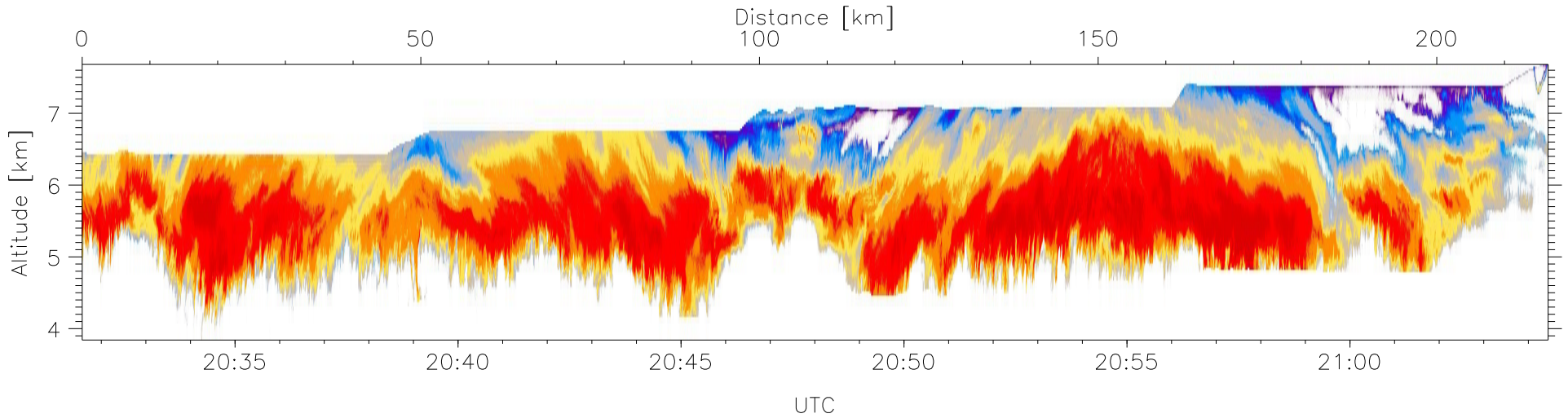
W2009-04-30-20-31-34: Down-slant Reflectivity
