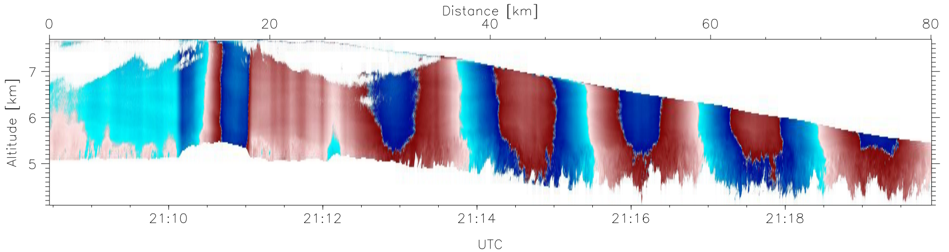
W2009-04-30-21-04-27: Down-slant Doppler
