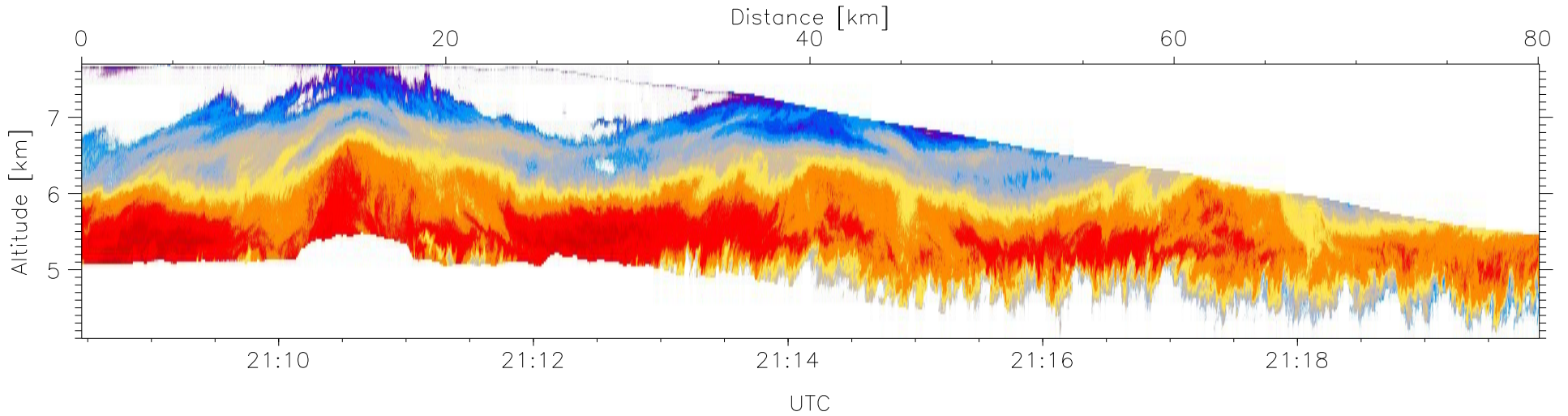
W2009-04-30-21-04-27: Down-slant Reflectivity
