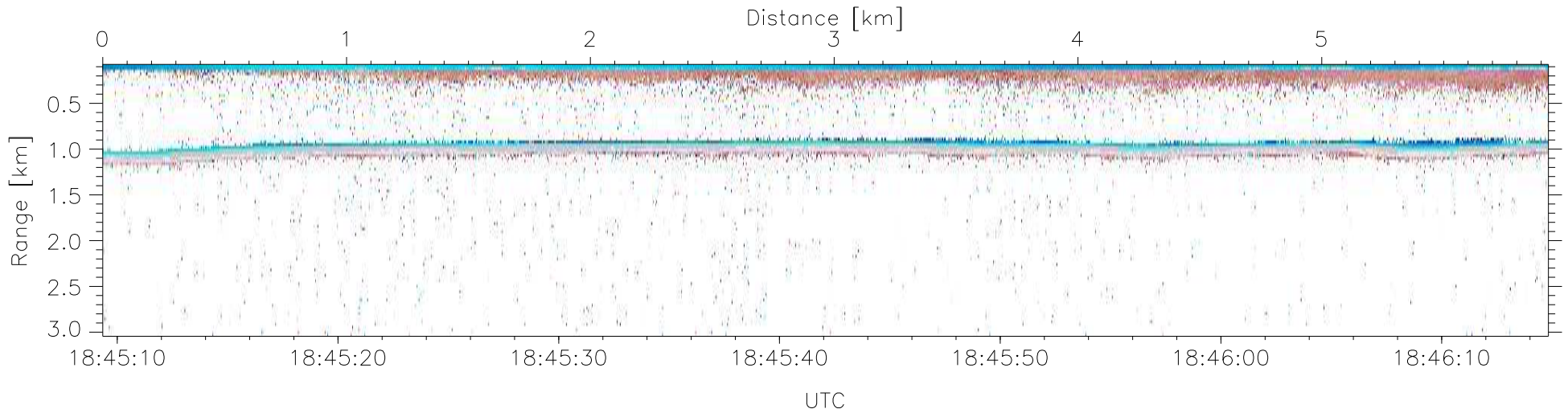
W2009-02-11-18-45-09: Down-slant Doppler
