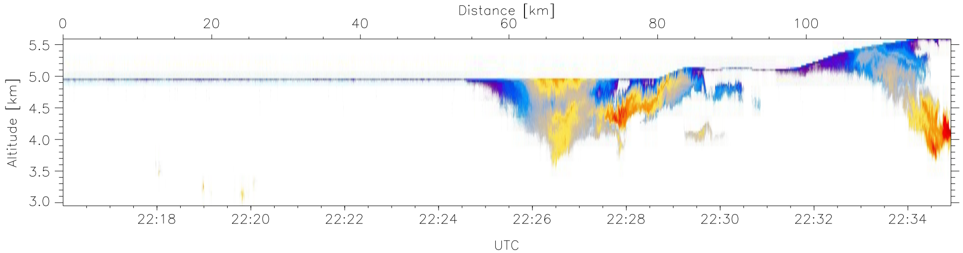
W2009-02-16-21-57-28: Down-slant Reflectivity
