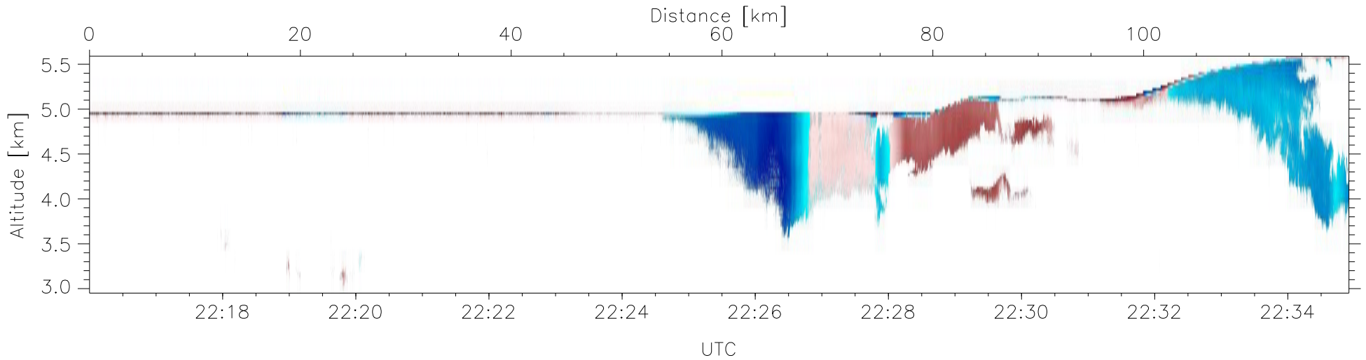
W2009-02-16-21-57-28: Down-slant Doppler
